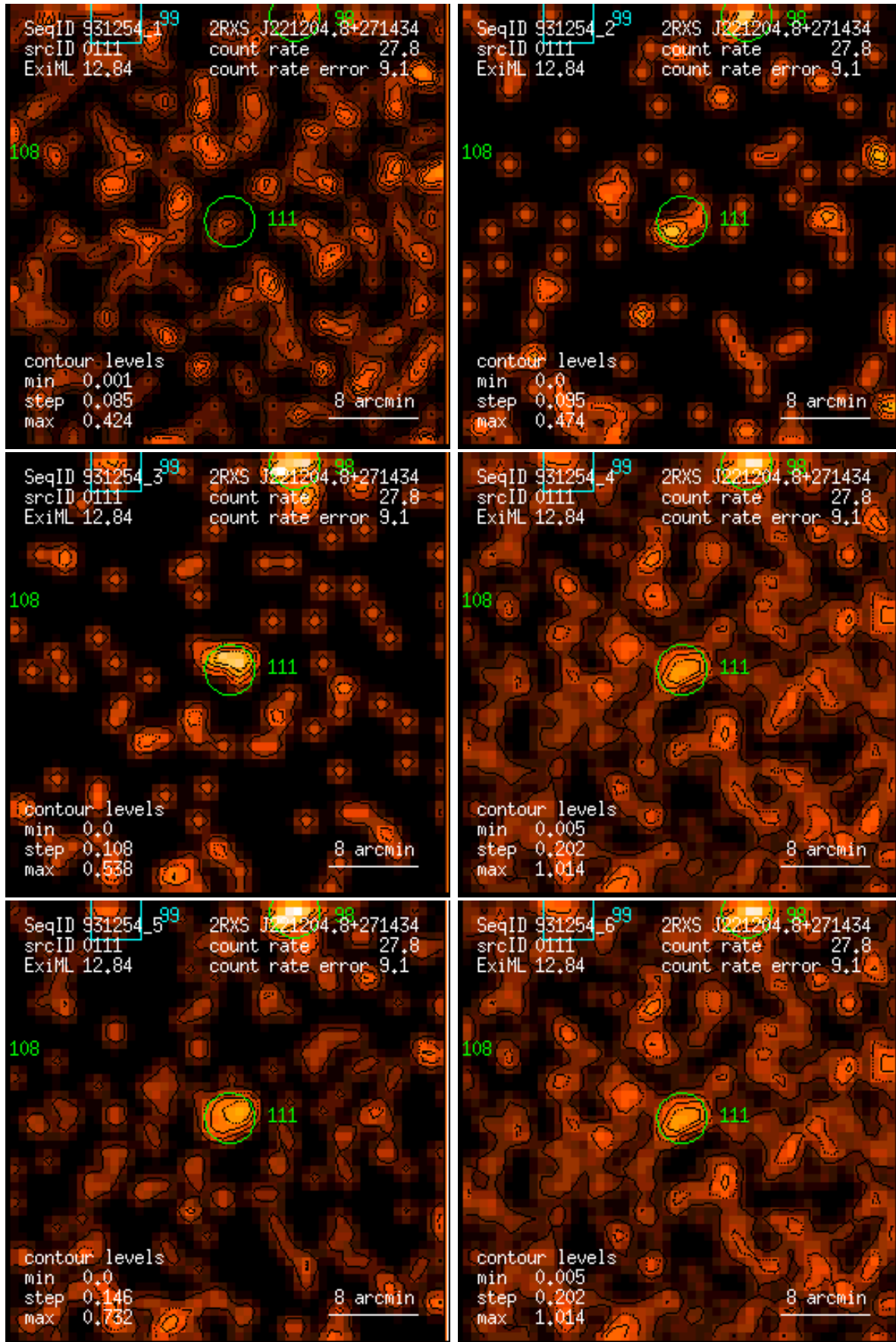
Figure 111: RASS 931254: detection 0111: band rate images, Gaussian filter: (1) PSPC channels 11 – 41, (2) 52 – 90, (3) 91 – 201, (4) 11 – 235, (5) 52 – 201, (6) 11 – 201. Broad band rates in counts/ks. Band rate contour levels in counts/ks/arcmin 2 .
