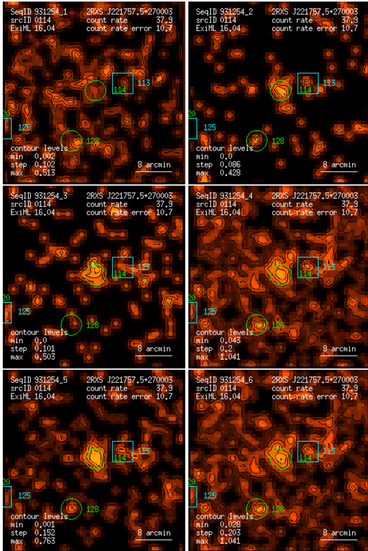
Figure 114: RASS 931254: detection 0114: band rate images, Gaussian filter: (1) PSPC channels 11 – 41, (2) 52 – 90, (3) 91 – 201, (4) 11 – 235, (5) 52 – 201, (6) 11 – 201. Broad band rates in counts/ks. Band rate contour levels in counts/ks/arcmin 2 .
