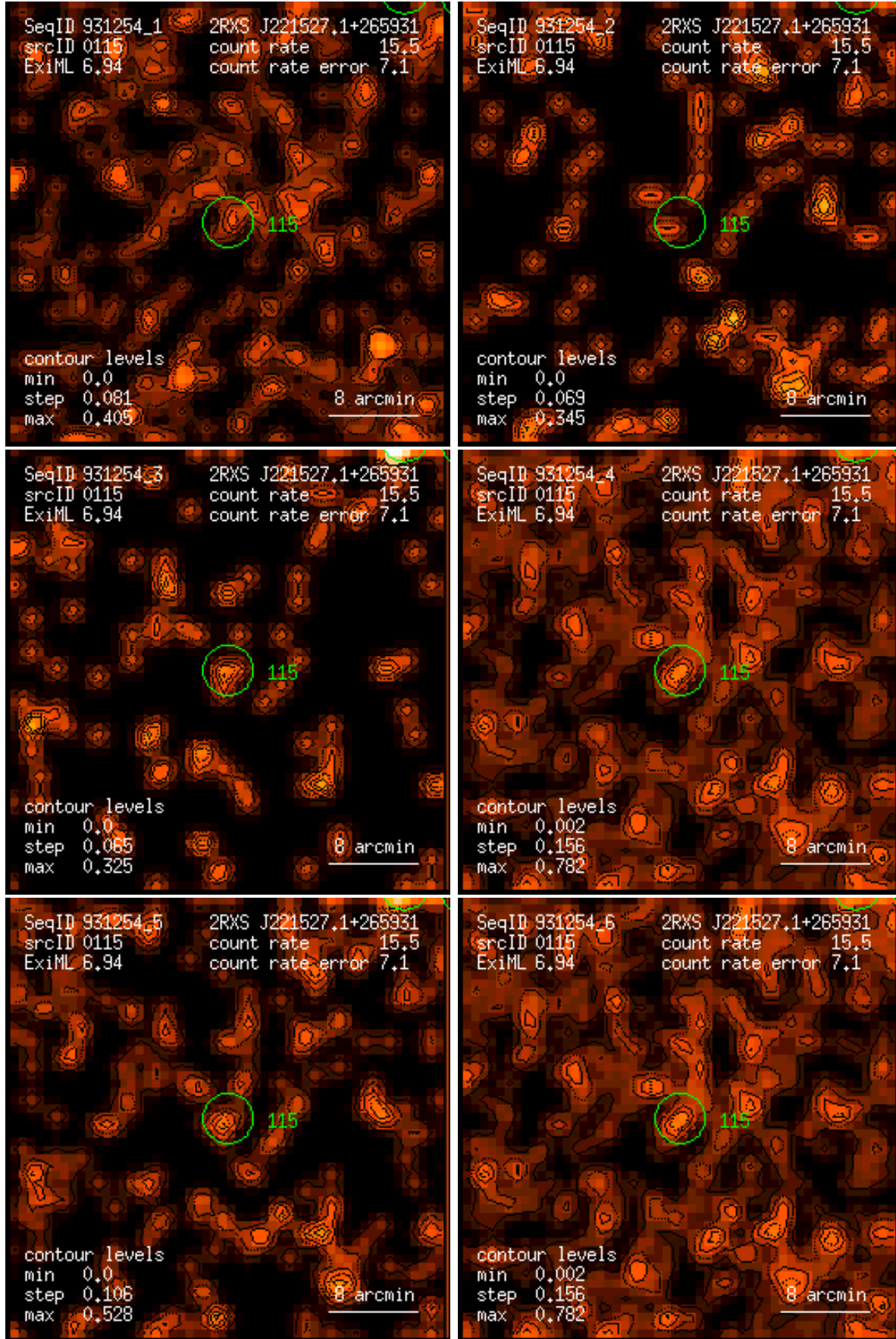
Figure 115: RASS 931254: detection 0115: band rate images, Gaussian filter: (1) PSPC channels 11 – 41, (2) 52 – 90, (3) 91 – 201, (4) 11 – 235, (5) 52 – 201, (6) 11 – 201. Broad band rates in counts/ks. Band rate contour levels in counts/ks/arcmin 2 .
