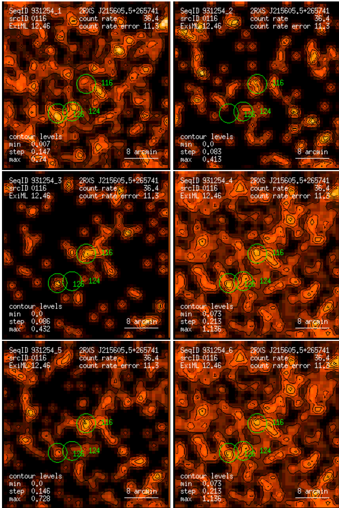
Figure 116: RASS 931254: detection 0116: band rate images, Gaussian filter: (1) PSPC channels 11 – 41, (2) 52 – 90, (3) 91 – 201, (4) 11 – 235, (5) 52 – 201, (6) 11 – 201. Broad band rates in counts/ks. Band rate contour levels in counts/ks/arcmin 2 .
