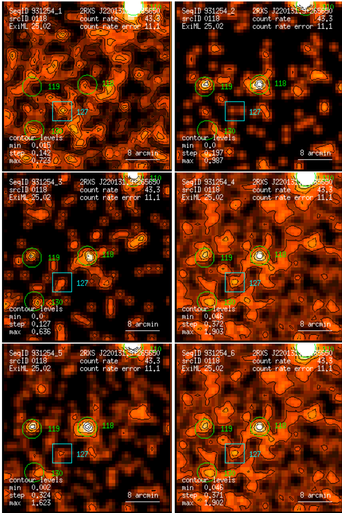
Figure 118: RASS 931254: detection 0118: band rate images, Gaussian filter: (1) PSPC channels 11 – 41, (2) 52 – 90, (3) 91 – 201, (4) 11 – 235, (5) 52 – 201, (6) 11 – 201. Broad band rates in counts/ks. Band rate contour levels in counts/ks/arcmin 2 .
