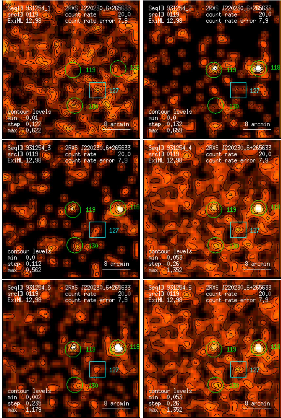
Figure 119: RASS 931254: detection 0119: band rate images, Gaussian filter: (1) PSPC channels 11 – 41, (2) 52 – 90, (3) 91 – 201, (4) 11 – 235, (5) 52 – 201, (6) 11 – 201. Broad band rates in counts/ks. Band rate contour levels in counts/ks/arcmin 2 .
