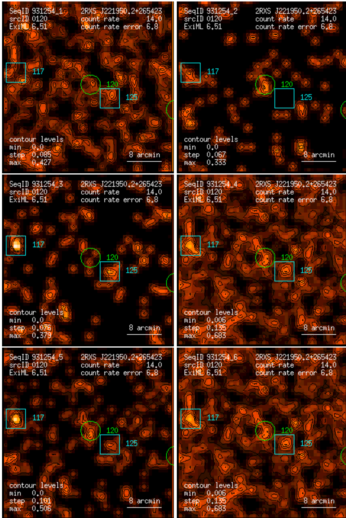
Figure 120: RASS 931254: detection 0120: band rate images, Gaussian filter: (1) PSPC channels 11 – 41, (2) 52 – 90, (3) 91 – 201, (4) 11 – 235, (5) 52 – 201, (6) 11 – 201. Broad band rates in counts/ks. Band rate contour levels in counts/ks/arcmin 2 .
