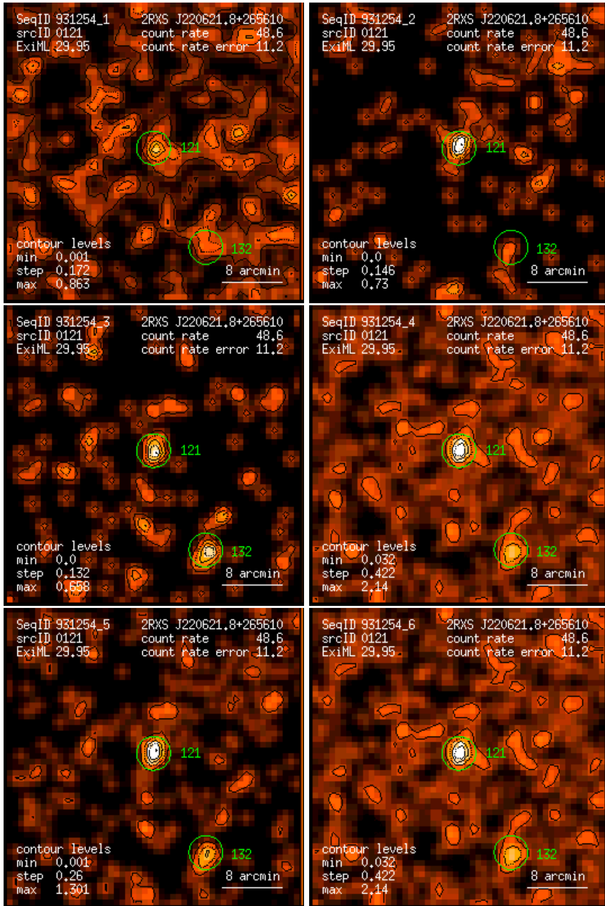
Figure 121: RASS 931254: detection 0121: band rate images, Gaussian filter: (1) PSPC channels 11 – 41, (2) 52 – 90, (3) 91 – 201, (4) 11 – 235, (5) 52 – 201, (6) 11 – 201. Broad band rates in counts/ks. Band rate contour levels in counts/ks/arcmin 2 .
