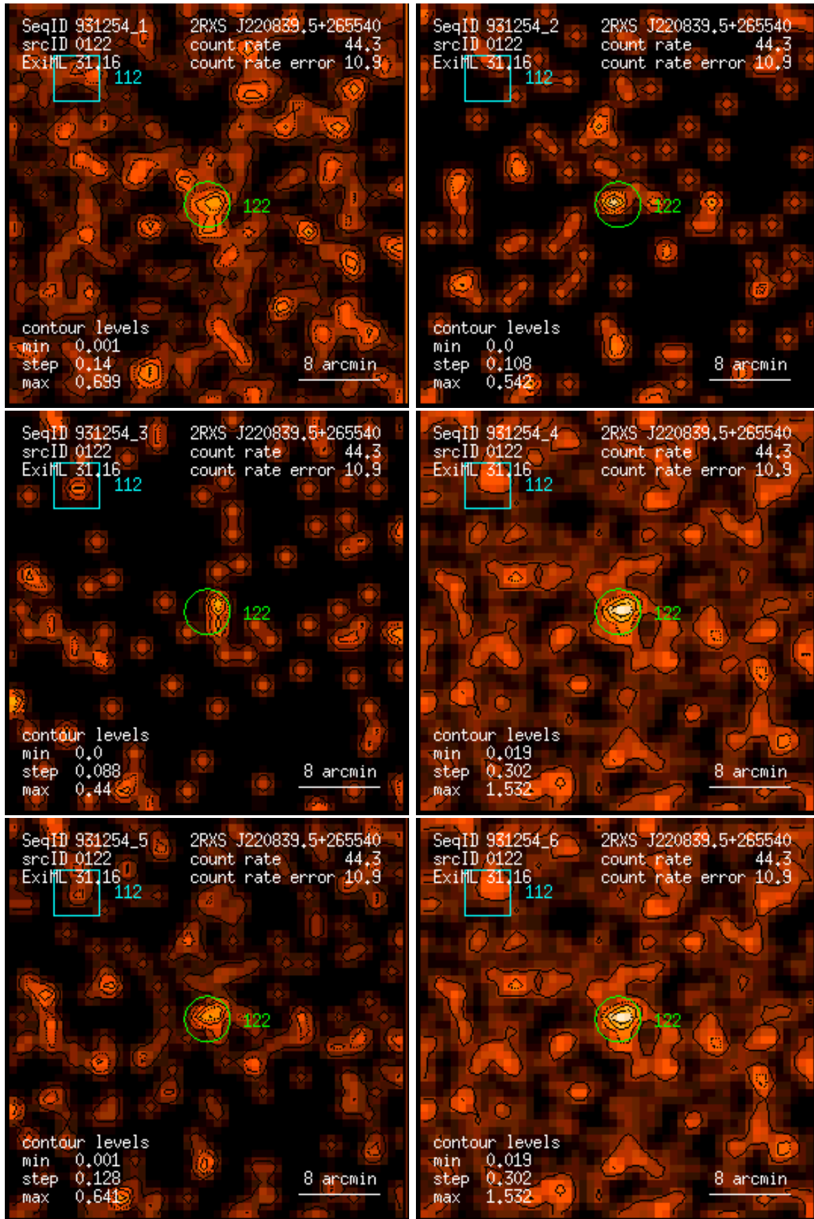
Figure 122: RASS 931254: detection 0122: band rate images, Gaussian filter: (1) PSPC channels 11 – 41, (2) 52 – 90, (3) 91 – 201, (4) 11 – 235, (5) 52 – 201, (6) 11 – 201. Broad band rates in counts/ks. Band rate contour levels in counts/ks/arcmin 2 .
