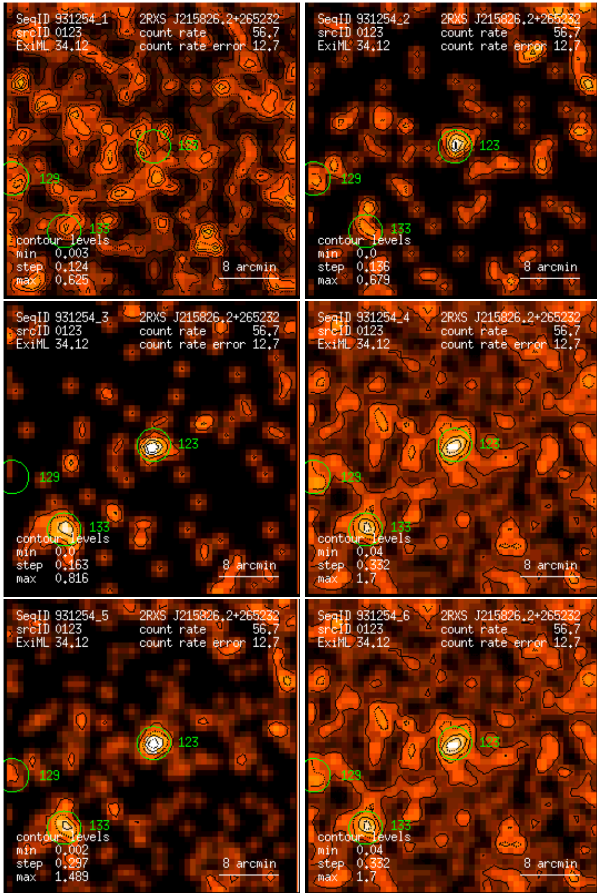
Figure 123: RASS 931254: detection 0123: band rate images, Gaussian filter: (1) PSPC channels 11 – 41, (2) 52 – 90, (3) 91 – 201, (4) 11 – 235, (5) 52 – 201, (6) 11 – 201. Broad band rates in counts/ks. Band rate contour levels in counts/ks/arcmin 2 .
