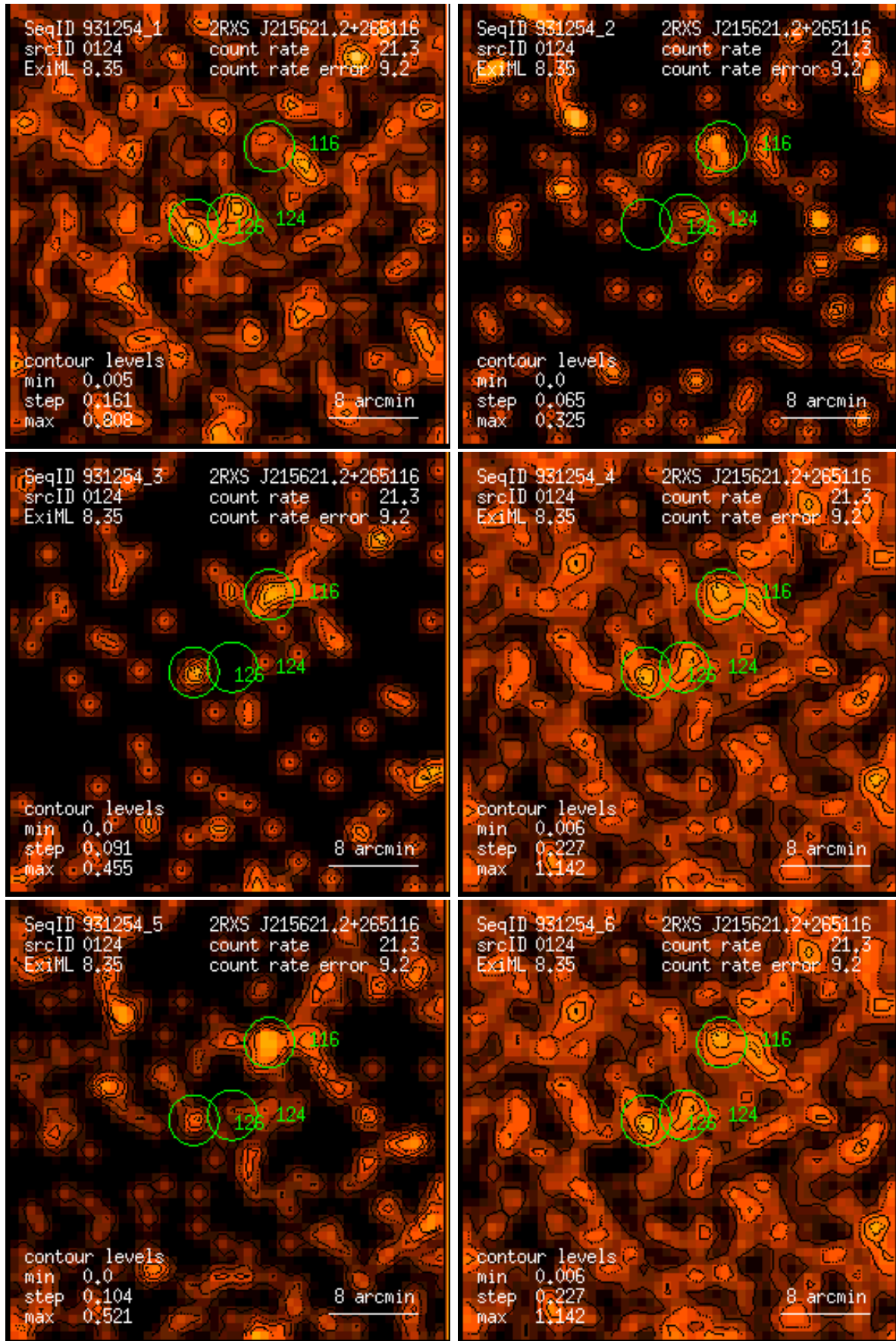
Figure 124: RASS 931254: detection 0124: band rate images, Gaussian filter: (1) PSPC channels 11 – 41, (2) 52 – 90, (3) 91 – 201, (4) 11 – 235, (5) 52 – 201, (6) 11 – 201. Broad band rates in counts/ks. Band rate contour levels in counts/ks/arcmin 2 .
