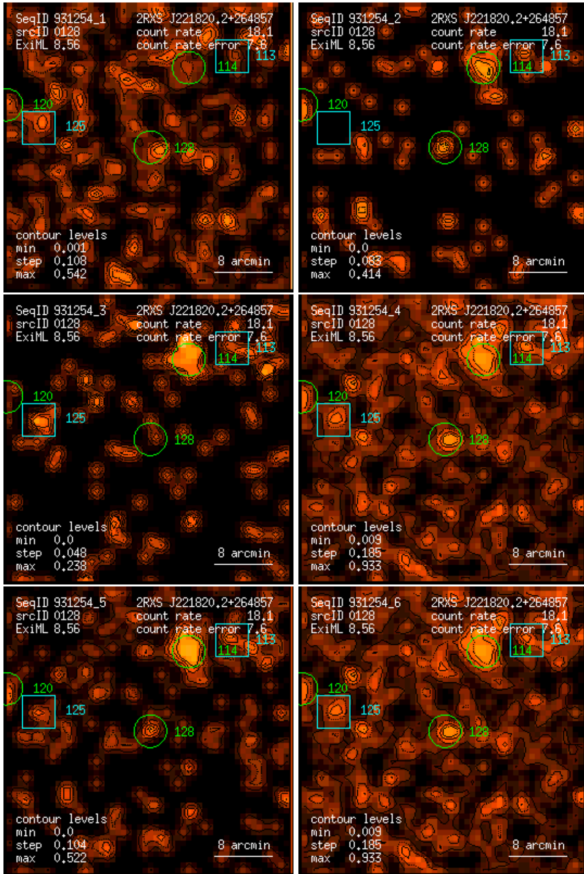
Figure 128: RASS 931254: detection 0128: band rate images, Gaussian filter: (1) PSPC channels 11 – 41, (2) 52 – 90, (3) 91 – 201, (4) 11 – 235, (5) 52 – 201, (6) 11 – 201. Broad band rates in counts/ks. Band rate contour levels in counts/ks/arcmin 2 .
