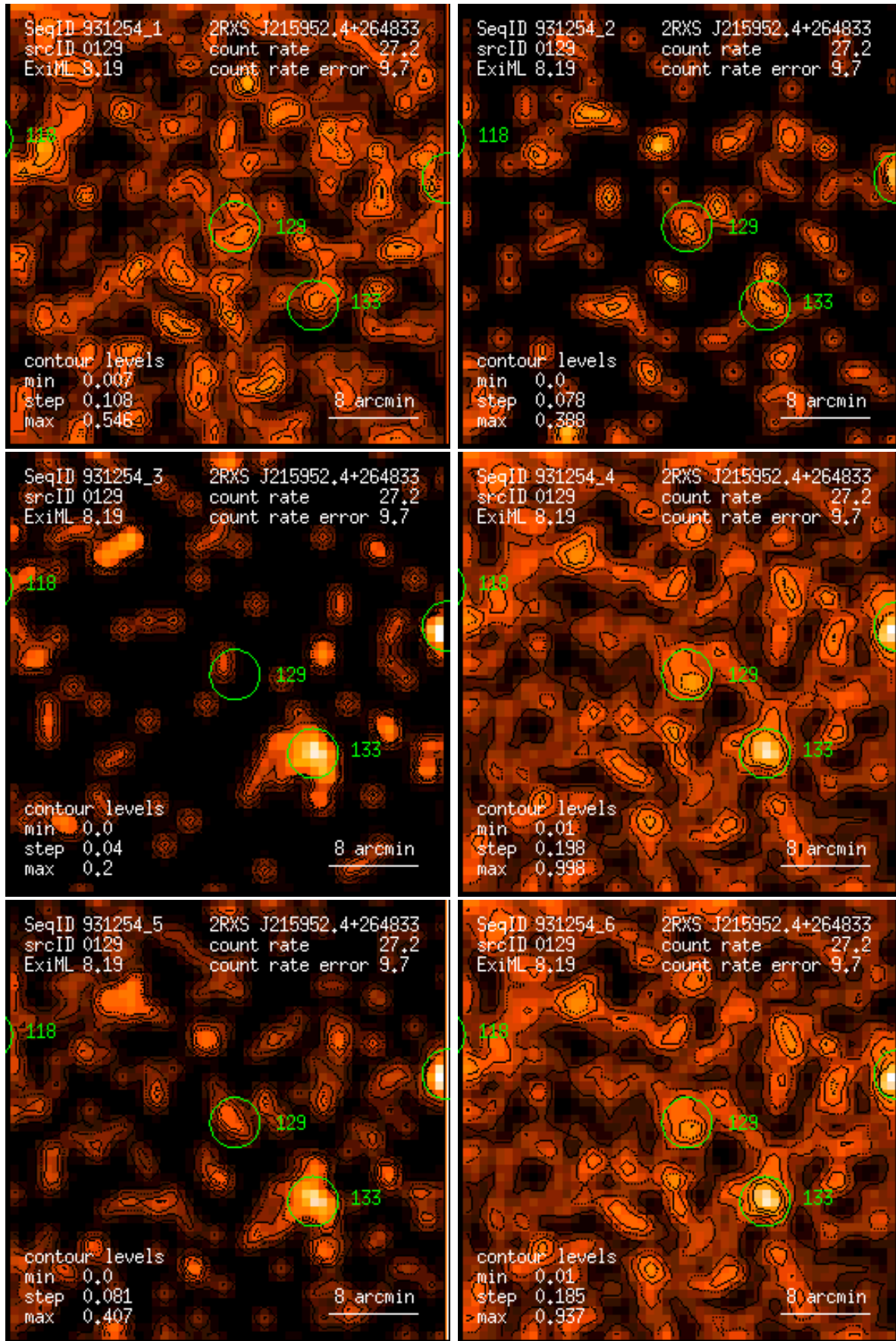
Figure 129: RASS 931254: detection 0129: band rate images, Gaussian filter: (1) PSPC channels 11 – 41, (2) 52 – 90, (3) 91 – 201, (4) 11 – 235, (5) 52 – 201, (6) 11 – 201. Broad band rates in counts/ks. Band rate contour levels in counts/ks/arcmin 2 .
