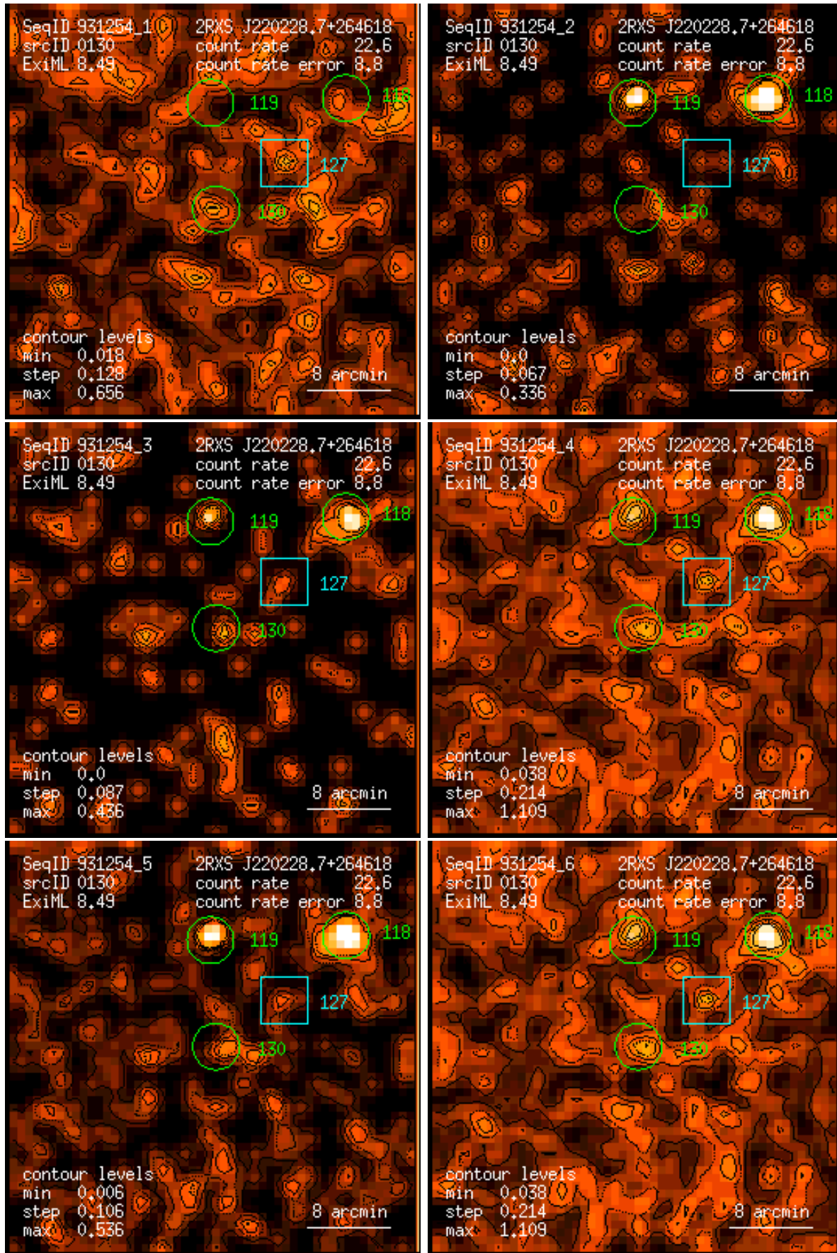
Figure 130: RASS 931254: detection 0130: band rate images, Gaussian filter: (1) PSPC channels 11 – 41, (2) 52 – 90, (3) 91 – 201, (4) 11 – 235, (5) 52 – 201, (6) 11 – 201. Broad band rates in counts/ks. Band rate contour levels in counts/ks/arcmin 2 .
