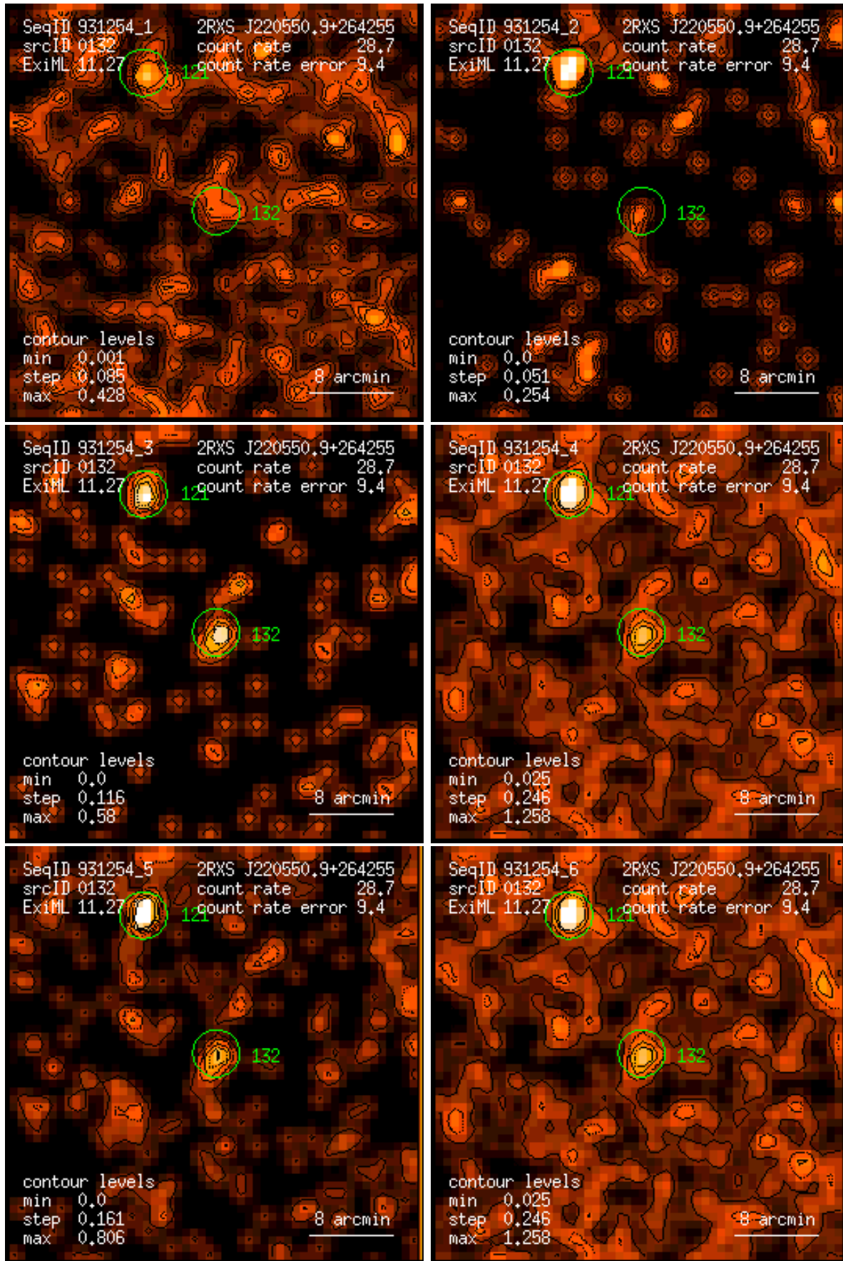
Figure 132: RASS 931254: detection 0132: band rate images, Gaussian filter: (1) PSPC channels 11 – 41, (2) 52 – 90, (3) 91 – 201, (4) 11 – 235, (5) 52 – 201, (6) 11 – 201. Broad band rates in counts/ks. Band rate contour levels in counts/ks/arcmin 2 .
