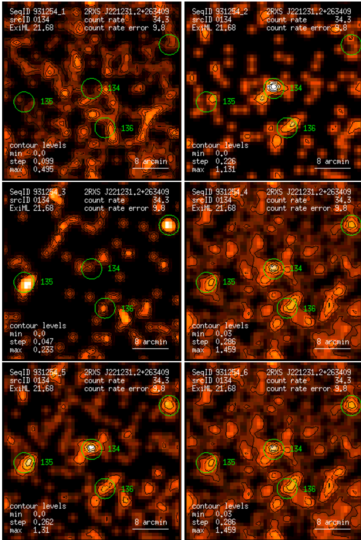
Figure 134: RASS 931254: detection 0134: band rate images, Gaussian filter: (1) PSPC channels 11 – 41, (2) 52 – 90, (3) 91 – 201, (4) 11 – 235, (5) 52 – 201, (6) 11 – 201. Broad band rates in counts/ks. Band rate contour levels in counts/ks/arcmin 2 .
