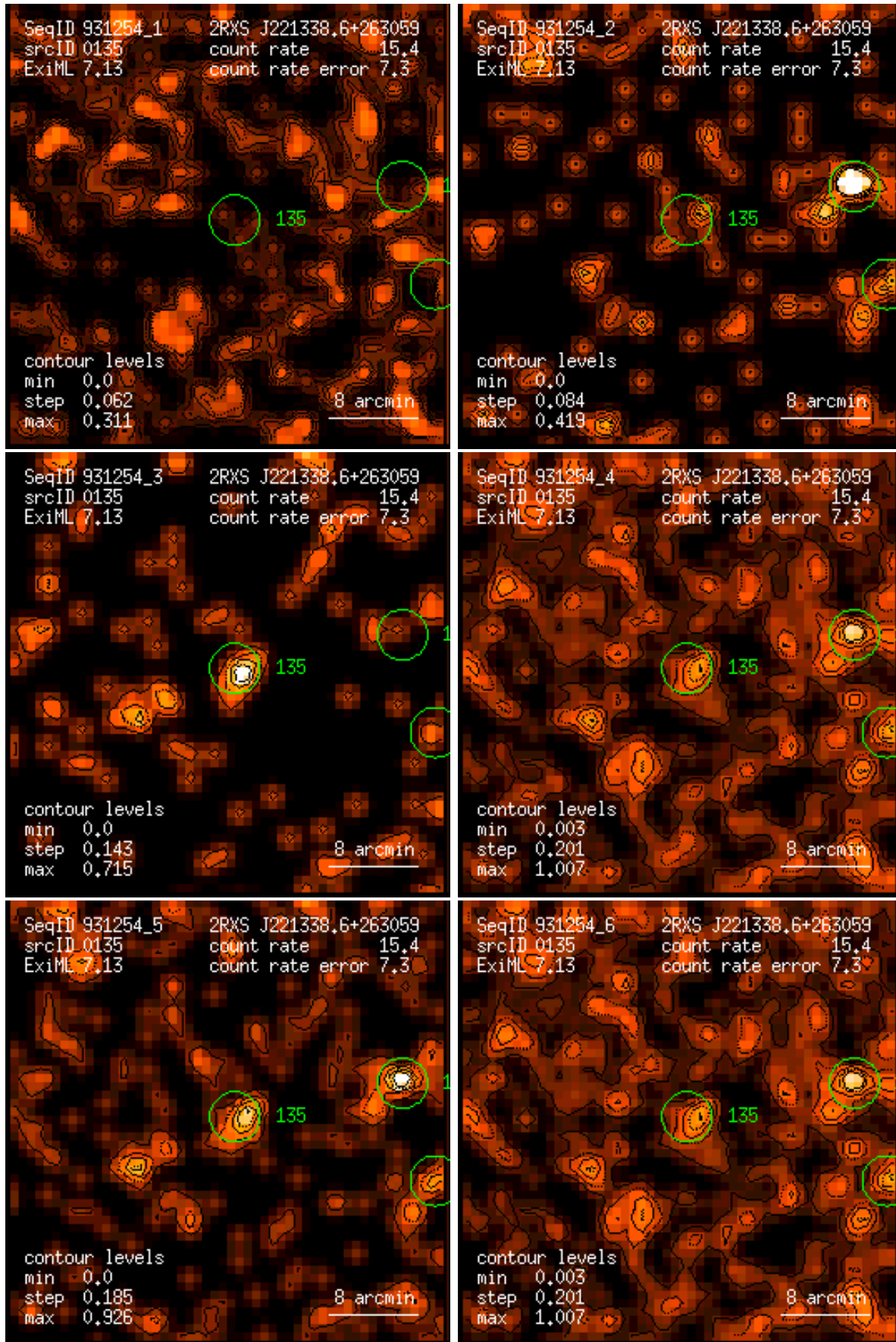
Figure 135: RASS 931254: detection 0135: band rate images, Gaussian filter: (1) PSPC channels 11 – 41, (2) 52 – 90, (3) 91 – 201, (4) 11 – 235, (5) 52 – 201, (6) 11 – 201. Broad band rates in counts/ks. Band rate contour levels in counts/ks/arcmin 2 .
