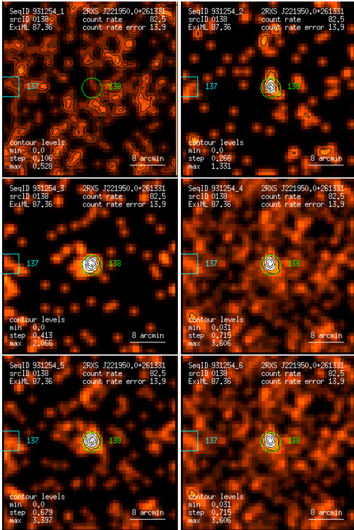
Figure 138: RASS 931254: detection 0138: band rate images, Gaussian filter: (1) PSPC channels 11 – 41, (2) 52 – 90, (3) 91 – 201, (4) 11 – 235, (5) 52 – 201, (6) 11 – 201. Broad band rates in counts/ks. Band rate contour levels in counts/ks/arcmin 2 .
