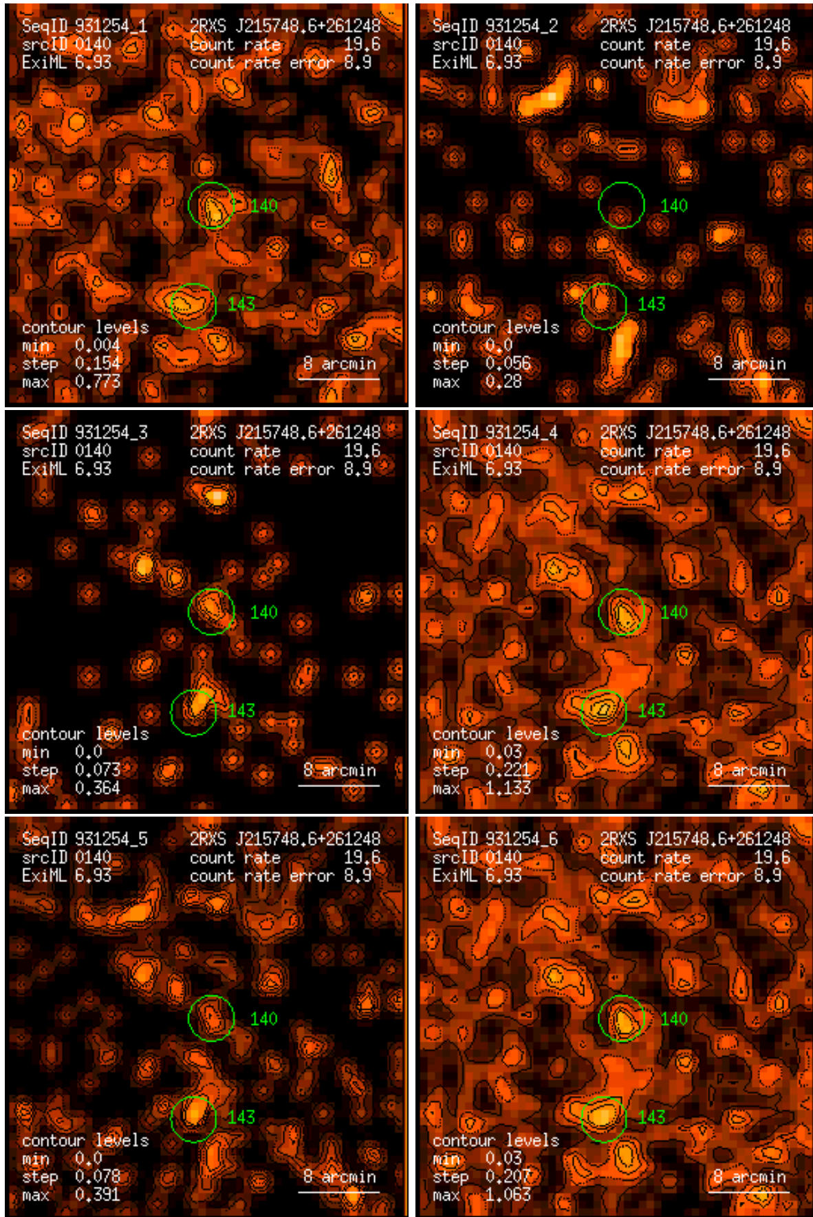
Figure 140: RASS 931254: detection 0140: band rate images, Gaussian filter: (1) PSPC channels 11 – 41, (2) 52 – 90, (3) 91 – 201, (4) 11 – 235, (5) 52 – 201, (6) 11 – 201. Broad band rates in counts/ks. Band rate contour levels in counts/ks/arcmin 2 .
