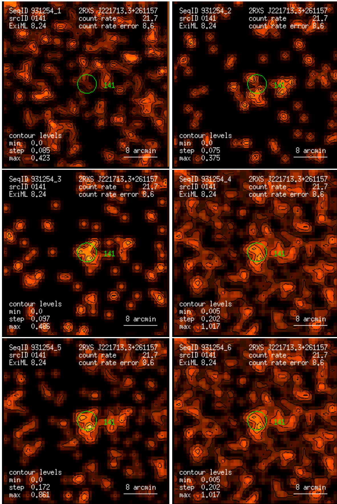
Figure 141: RASS 931254: detection 0141: band rate images, Gaussian filter: (1) PSPC channels 11 – 41, (2) 52 – 90, (3) 91 – 201, (4) 11 – 235, (5) 52 – 201, (6) 11 – 201. Broad band rates in counts/ks. Band rate contour levels in counts/ks/arcmin 2 .
