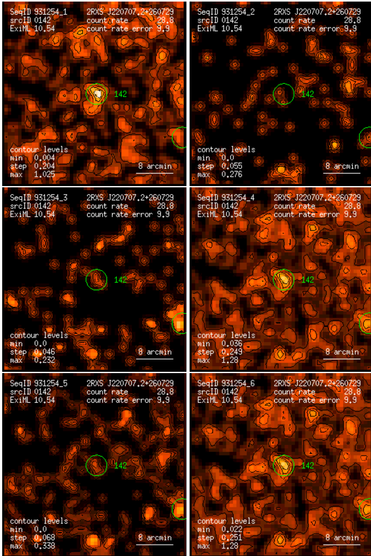
Figure 142: RASS 931254: detection 0142: band rate images, Gaussian filter: (1) PSPC channels 11 – 41, (2) 52 – 90, (3) 91 – 201, (4) 11 – 235, (5) 52 – 201, (6) 11 – 201. Broad band rates in counts/ks. Band rate contour levels in counts/ks/arcmin 2 .
