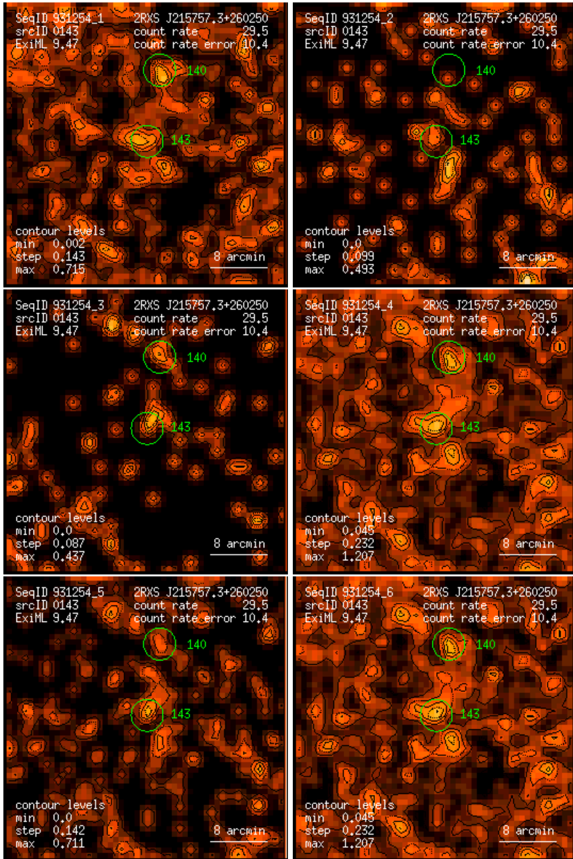
Figure 143: RASS 931254: detection 0143: band rate images, Gaussian filter: (1) PSPC channels 11 – 41, (2) 52 – 90, (3) 91 – 201, (4) 11 – 235, (5) 52 – 201, (6) 11 – 201. Broad band rates in counts/ks. Band rate contour levels in counts/ks/arcmin 2 .
