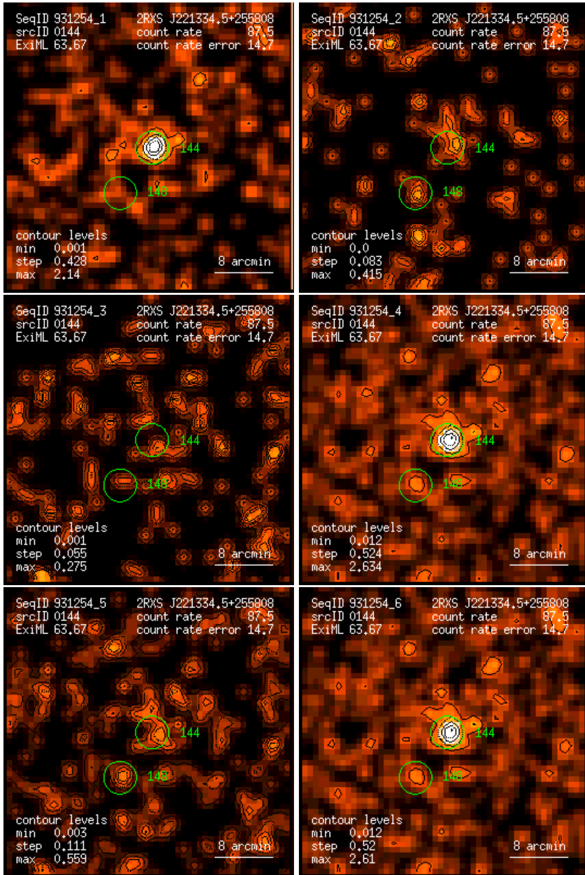
Figure 144: RASS 931254: detection 0144: band rate images, Gaussian filter: (1) PSPC channels 11 – 41, (2) 52 – 90, (3) 91 – 201, (4) 11 – 235, (5) 52 – 201, (6) 11 – 201. Broad band rates in counts/ks. Band rate contour levels in counts/ks/arcmin 2 .
