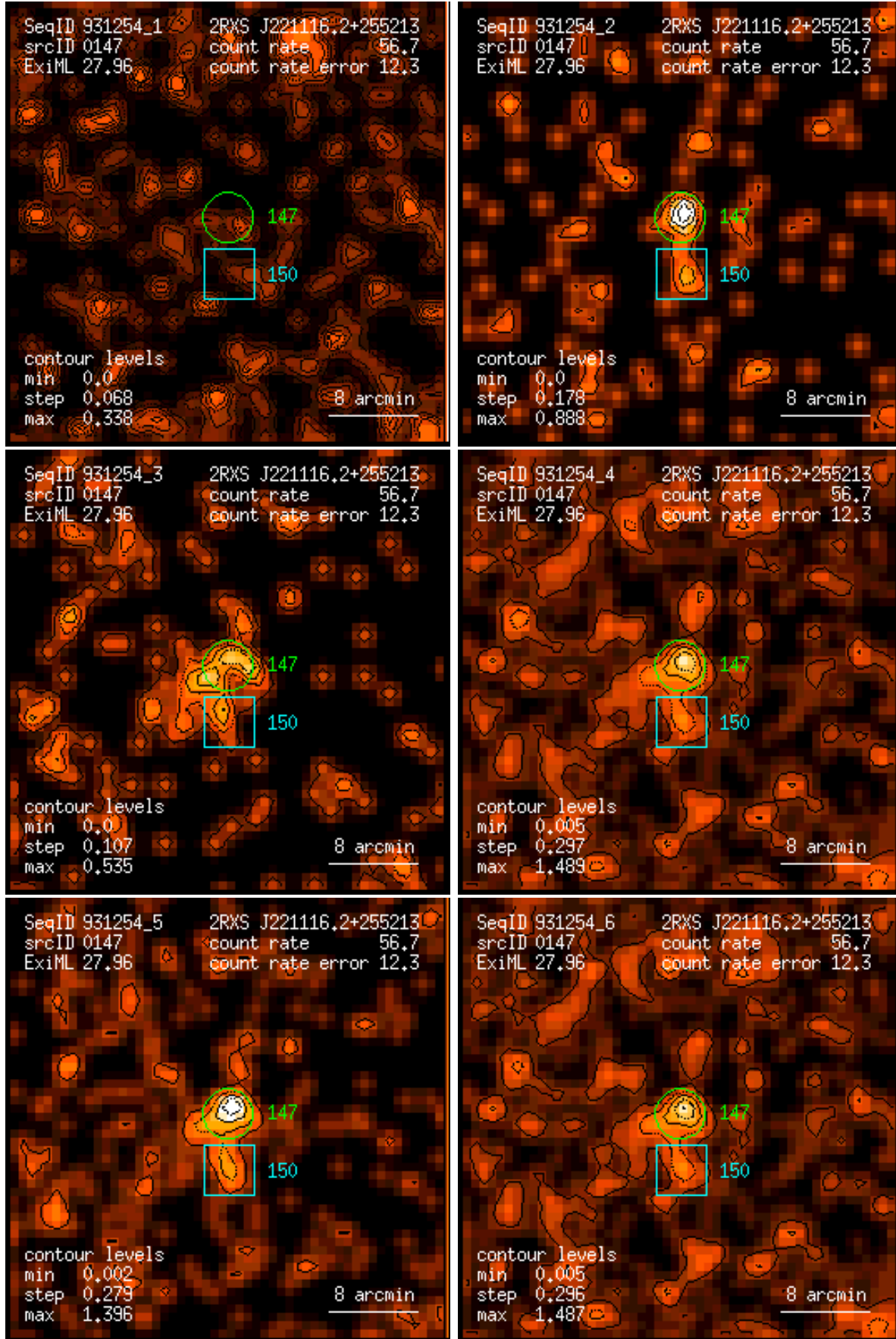
Figure 147: RASS 931254: detection 0147: band rate images, Gaussian filter: (1) PSPC channels 11 – 41, (2) 52 – 90, (3) 91 – 201, (4) 11 – 235, (5) 52 – 201, (6) 11 – 201. Broad band rates in counts/ks. Band rate contour levels in counts/ks/arcmin 2 .
