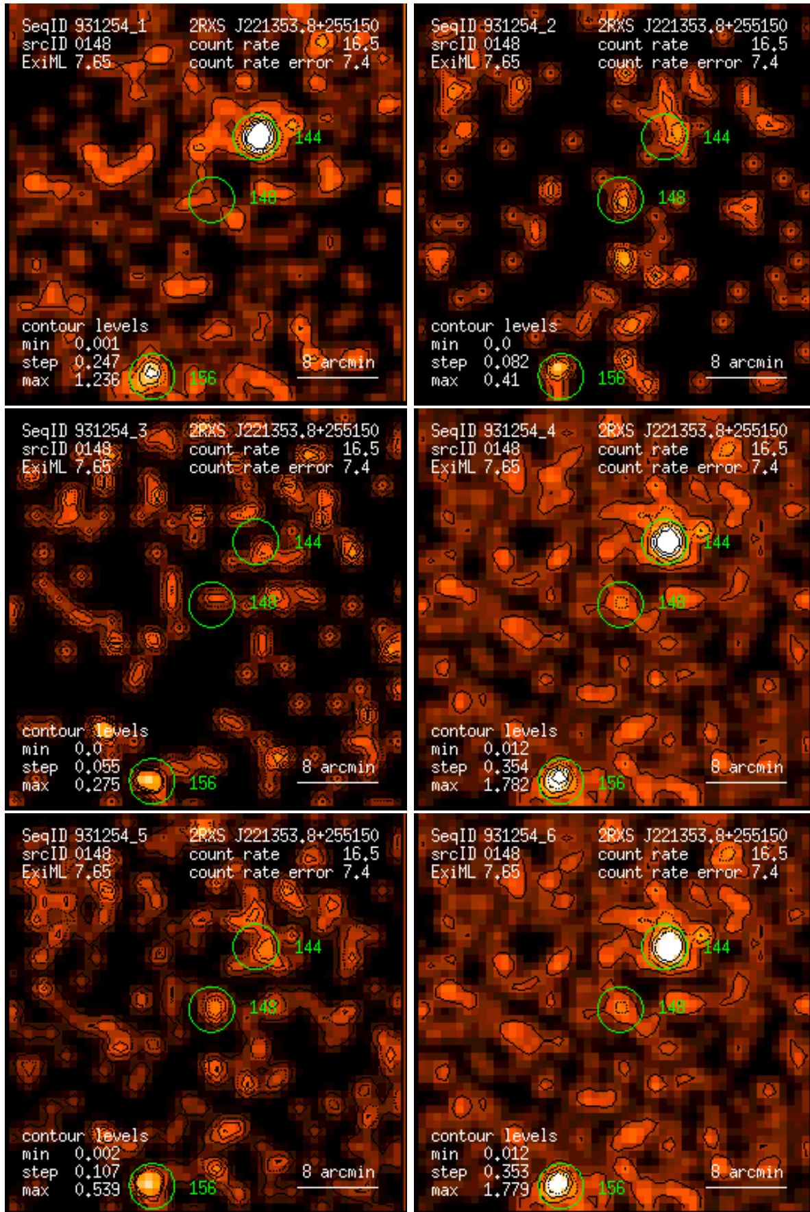
Figure 148: RASS 931254: detection 0148: band rate images, Gaussian filter: (1) PSPC channels 11 – 41, (2) 52 – 90, (3) 91 – 201, (4) 11 – 235, (5) 52 – 201, (6) 11 – 201. Broad band rates in counts/ks. Band rate contour levels in counts/ks/arcmin 2 .
