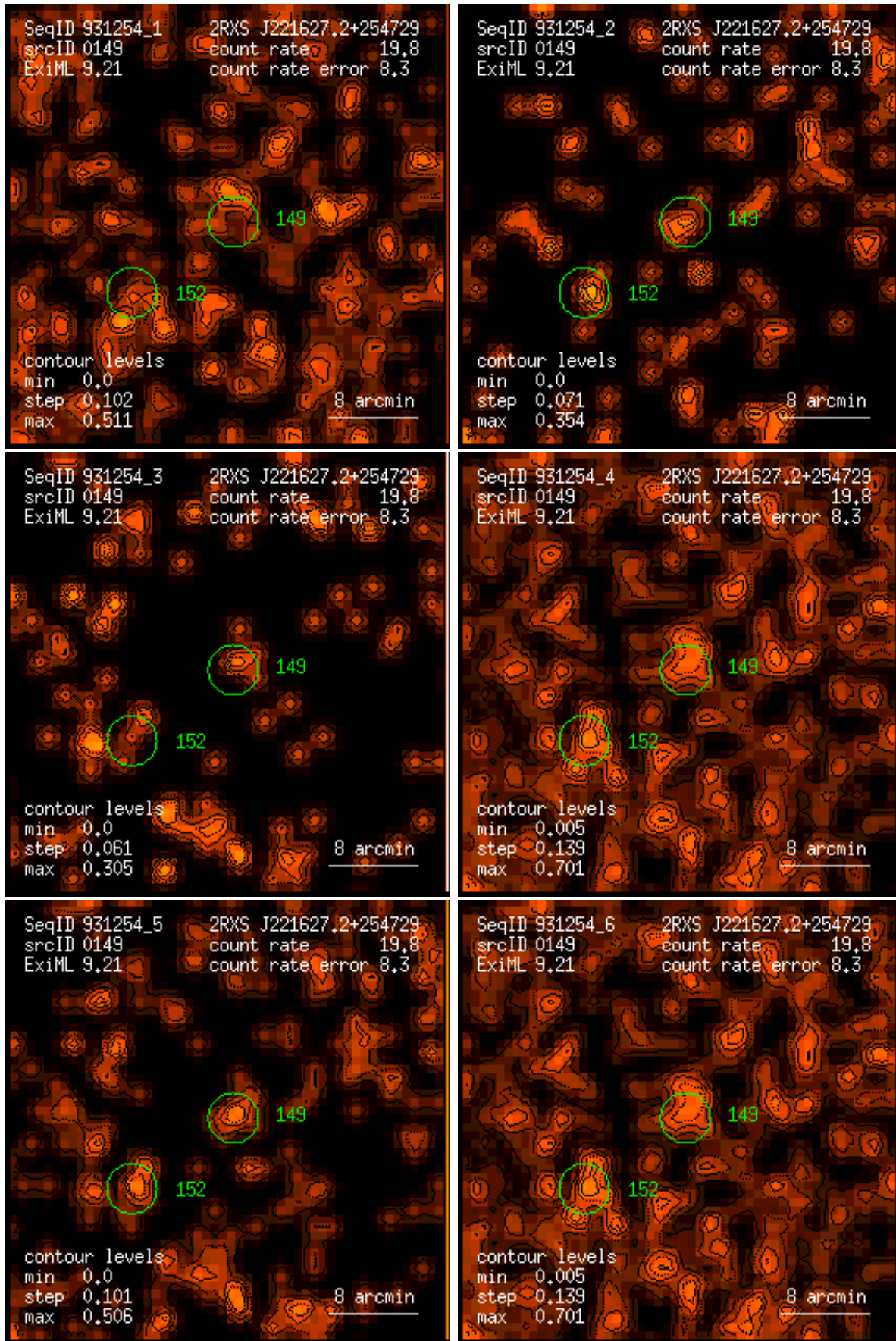
Figure 149: RASS 931254: detection 0149: band rate images, Gaussian filter: (1) PSPC channels 11 – 41, (2) 52 – 90, (3) 91 – 201, (4) 11 – 235, (5) 52 – 201, (6) 11 – 201. Broad band rates in counts/ks. Band rate contour levels in counts/ks/arcmin 2 .
