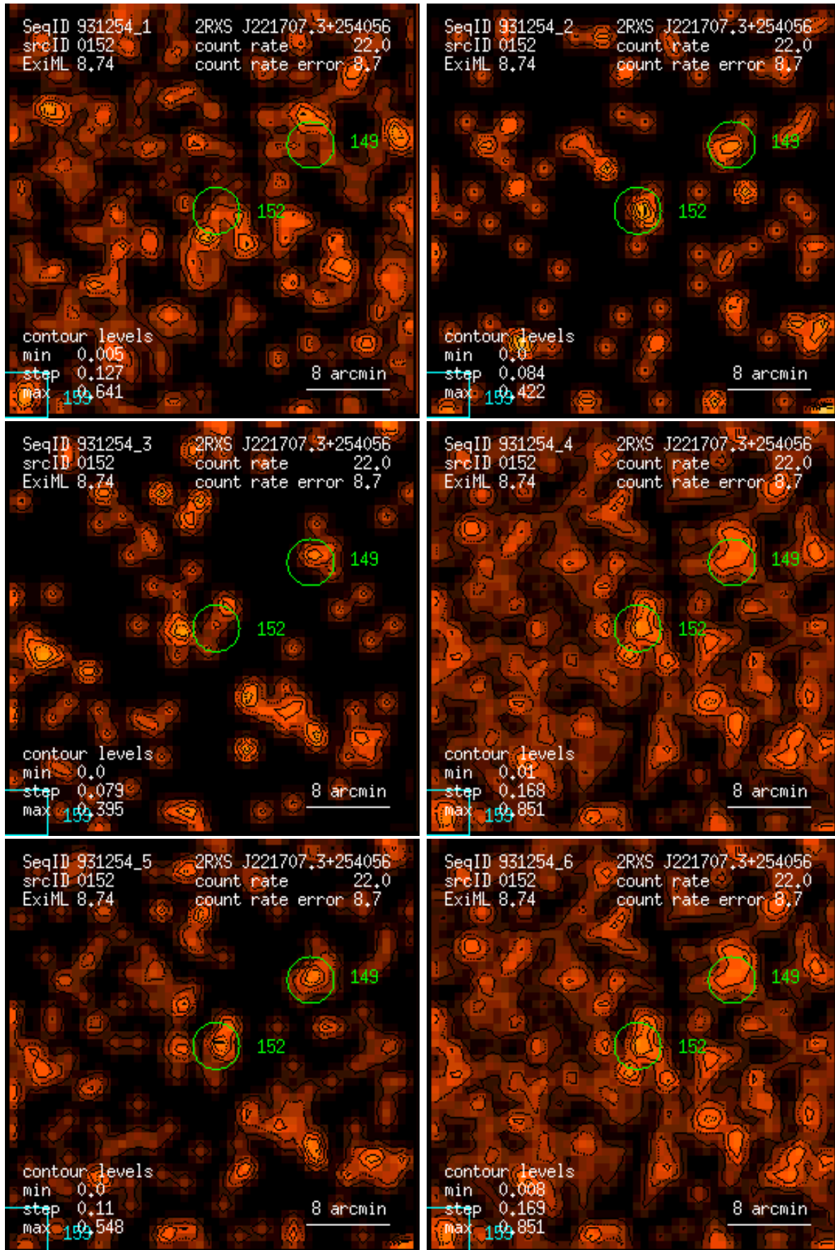
Figure 152: RASS 931254: detection 0152: band rate images, Gaussian filter: (1) PSPC channels 11 – 41, (2) 52 – 90, (3) 91 – 201, (4) 11 – 235, (5) 52 – 201, (6) 11 – 201. Broad band rates in counts/ks. Band rate contour levels in counts/ks/arcmin 2 .
