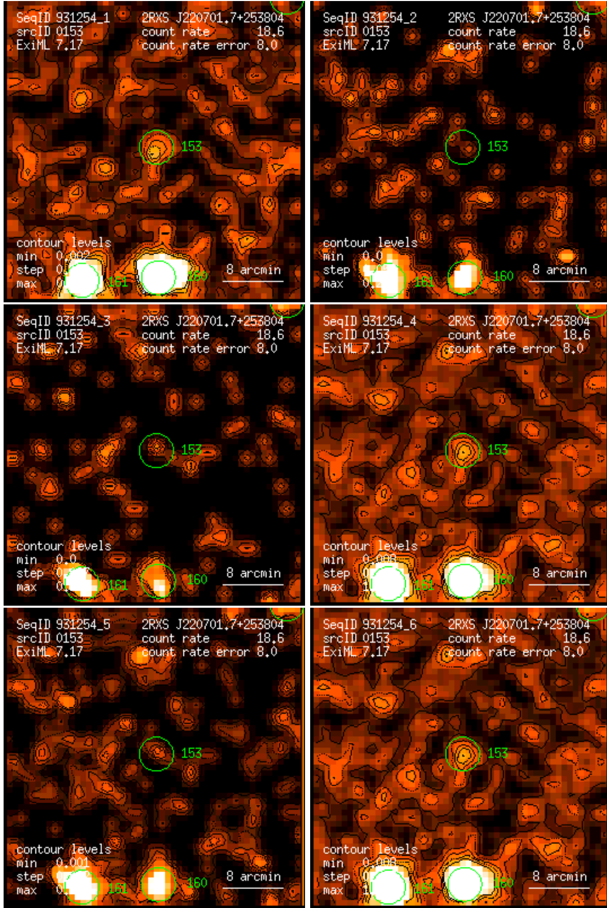
Figure 153: RASS 931254: detection 0153: band rate images, Gaussian filter: (1) PSPC channels 11 – 41, (2) 52 – 90, (3) 91 – 201, (4) 11 – 235, (5) 52 – 201, (6) 11 – 201. Broad band rates in counts/ks. Band rate contour levels in counts/ks/arcmin 2 .
