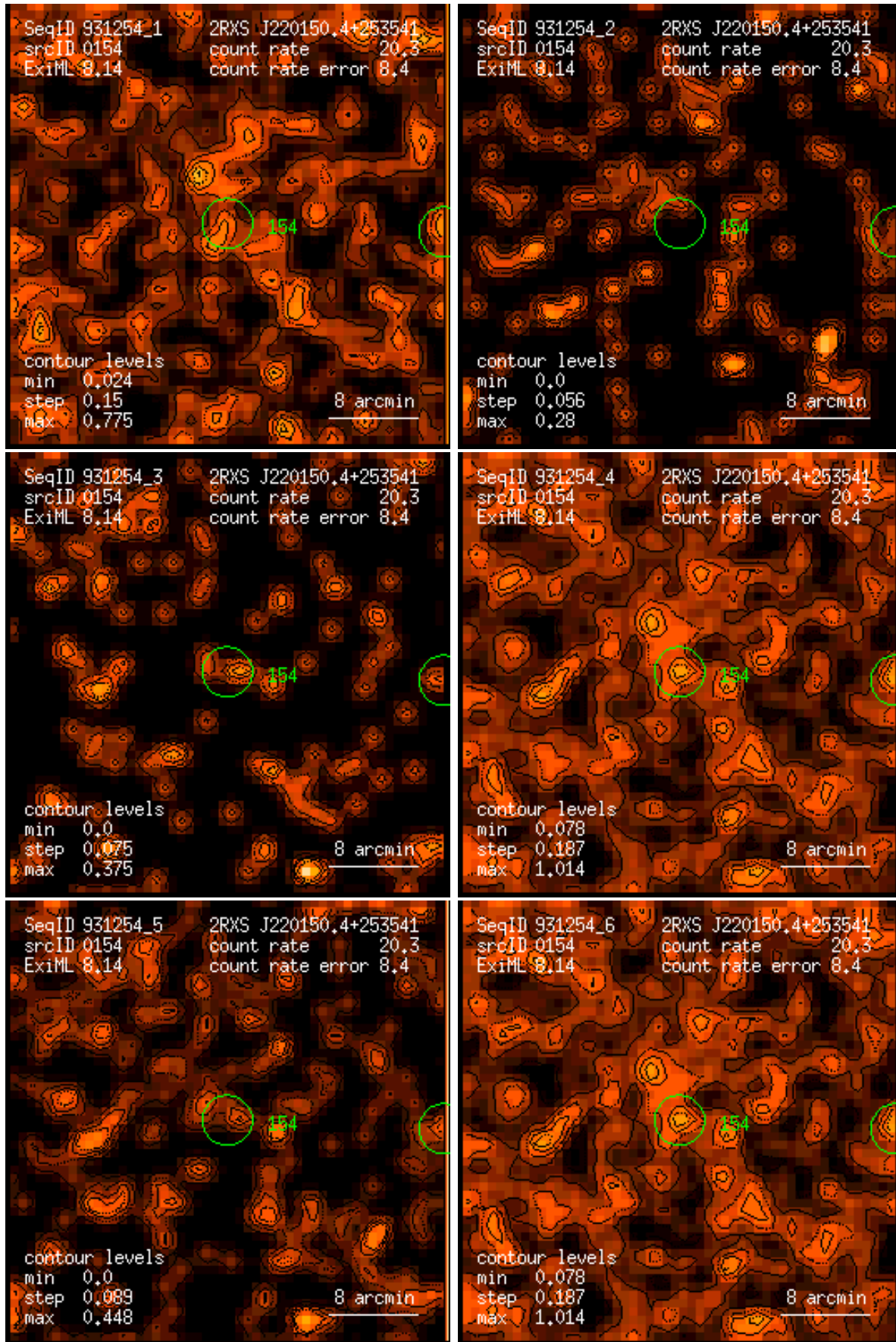
Figure 154: RASS 931254: detection 0154: band rate images, Gaussian filter: (1) PSPC channels 11 – 41, (2) 52 – 90, (3) 91 – 201, (4) 11 – 235, (5) 52 – 201, (6) 11 – 201. Broad band rates in counts/ks. Band rate contour levels in counts/ks/arcmin 2 .
