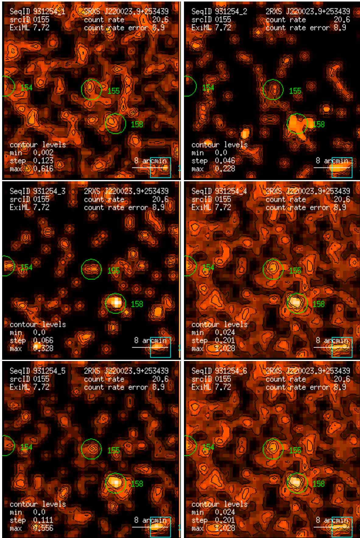
Figure 155: RASS 931254: detection 0155: band rate images, Gaussian filter: (1) PSPC channels 11 – 41, (2) 52 – 90, (3) 91 – 201, (4) 11 – 235, (5) 52 – 201, (6) 11 – 201. Broad band rates in counts/ks. Band rate contour levels in counts/ks/arcmin 2 .
