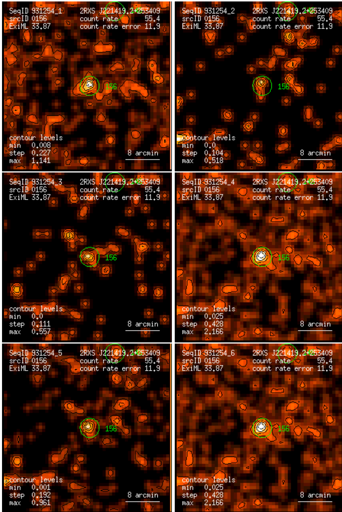
Figure 156: RASS 931254: detection 0156: band rate images, Gaussian filter: (1) PSPC channels 11 – 41, (2) 52 – 90, (3) 91 – 201, (4) 11 – 235, (5) 52 – 201, (6) 11 – 201. Broad band rates in counts/ks. Band rate contour levels in counts/ks/arcmin 2 .
