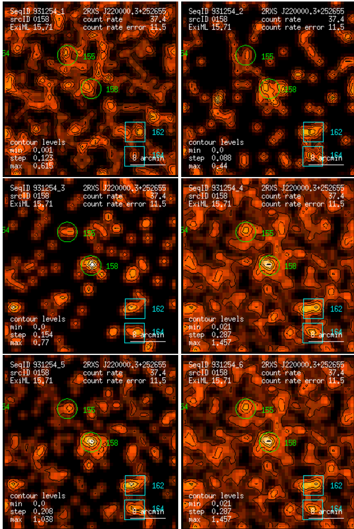
Figure 158: RASS 931254: detection 0158: band rate images, Gaussian filter: (1) PSPC channels 11 – 41, (2) 52 – 90, (3) 91 – 201, (4) 11 – 235, (5) 52 – 201, (6) 11 – 201. Broad band rates in counts/ks. Band rate contour levels in counts/ks/arcmin 2 .
