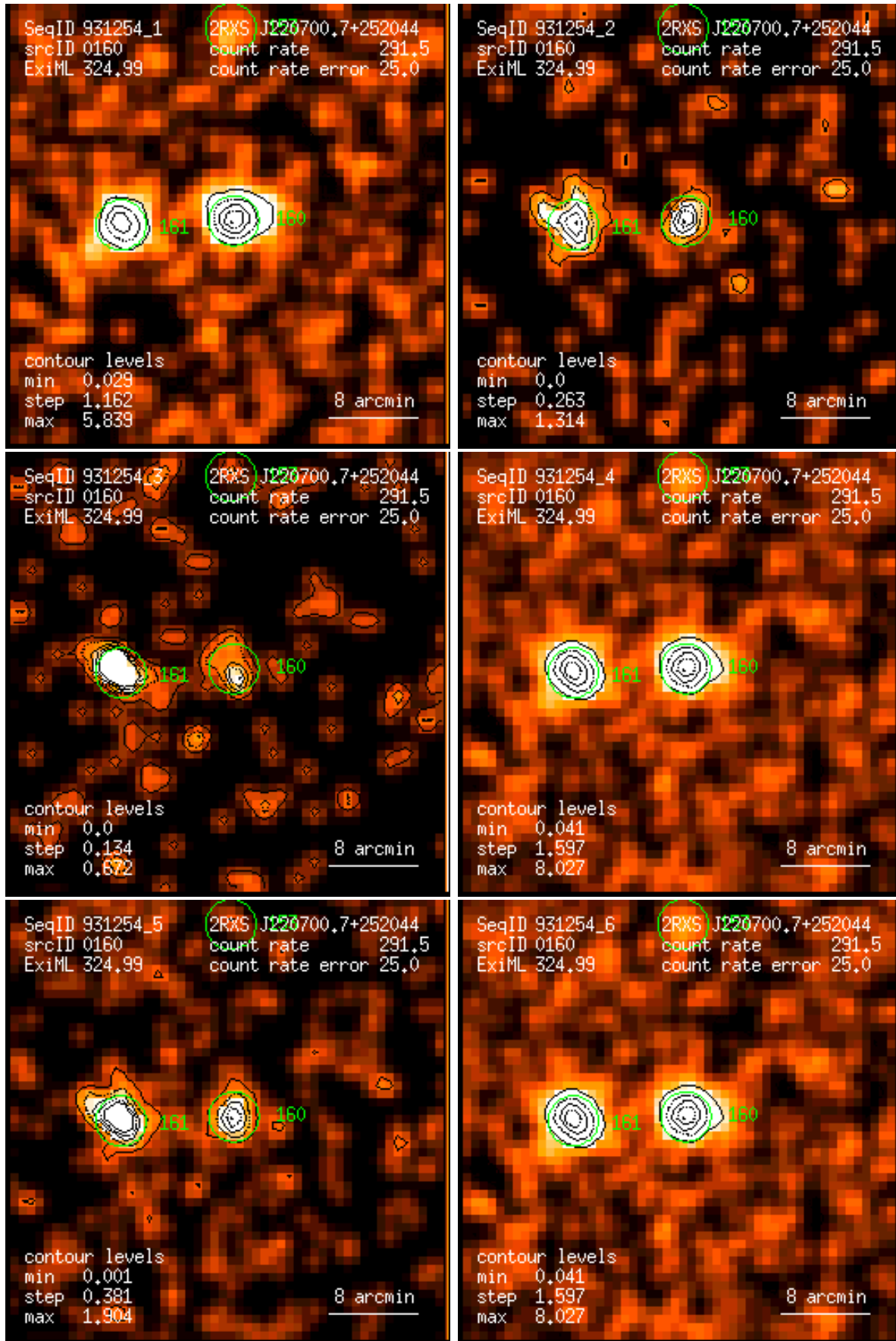
Figure 160: RASS 931254: detection 0160: band rate images, Gaussian filter: (1) PSPC channels 11 – 41, (2) 52 – 90, (3) 91 – 201, (4) 11 – 235, (5) 52 – 201, (6) 11 – 201. Broad band rates in counts/ks. Band rate contour levels in counts/ks/arcmin 2 .
