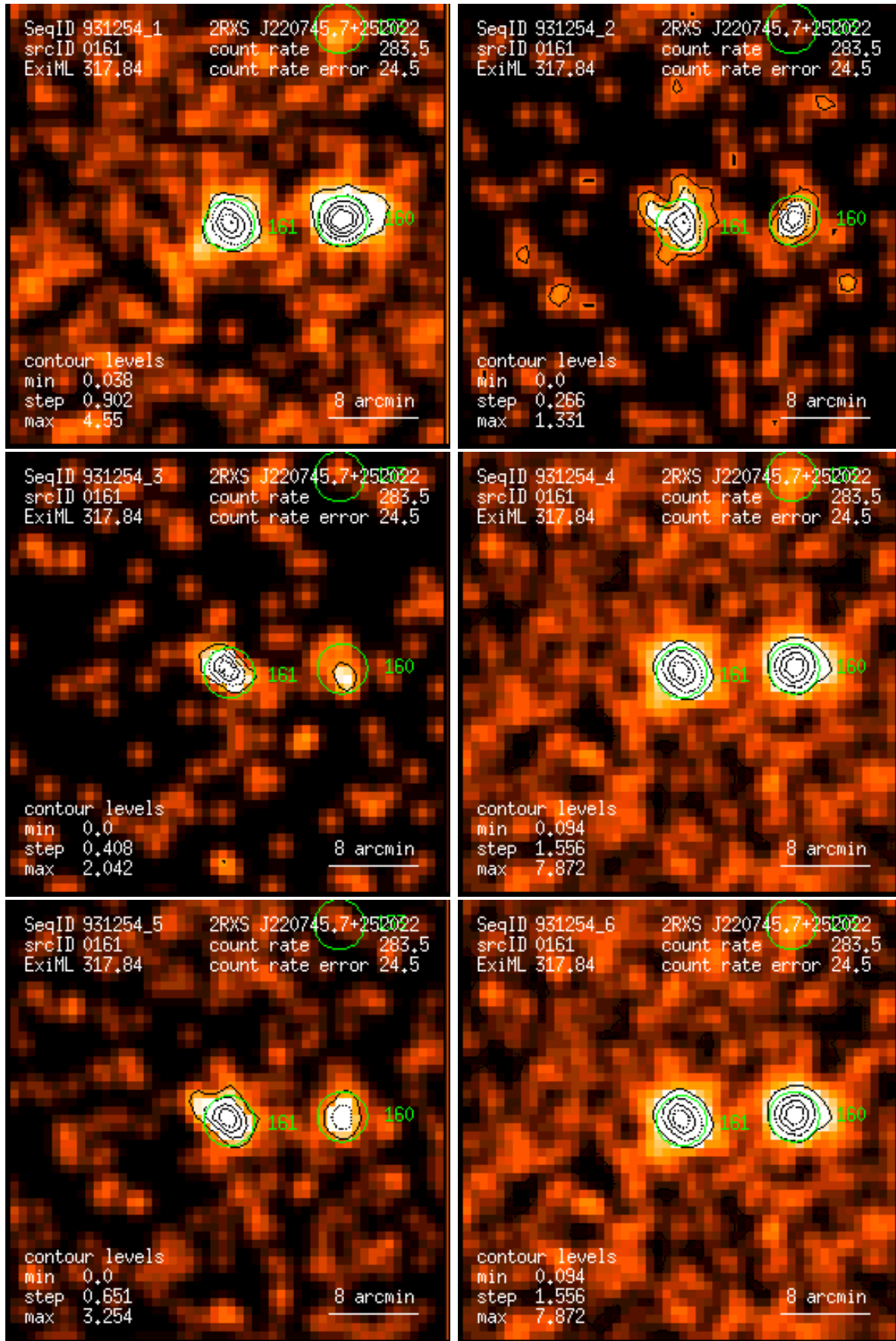
Figure 161: RASS 931254: detection 0161: band rate images, Gaussian filter: (1) PSPC channels 11 – 41, (2) 52 – 90, (3) 91 – 201, (4) 11 – 235, (5) 52 – 201, (6) 11 – 201. Broad band rates in counts/ks. Band rate contour levels in counts/ks/arcmin 2 .
