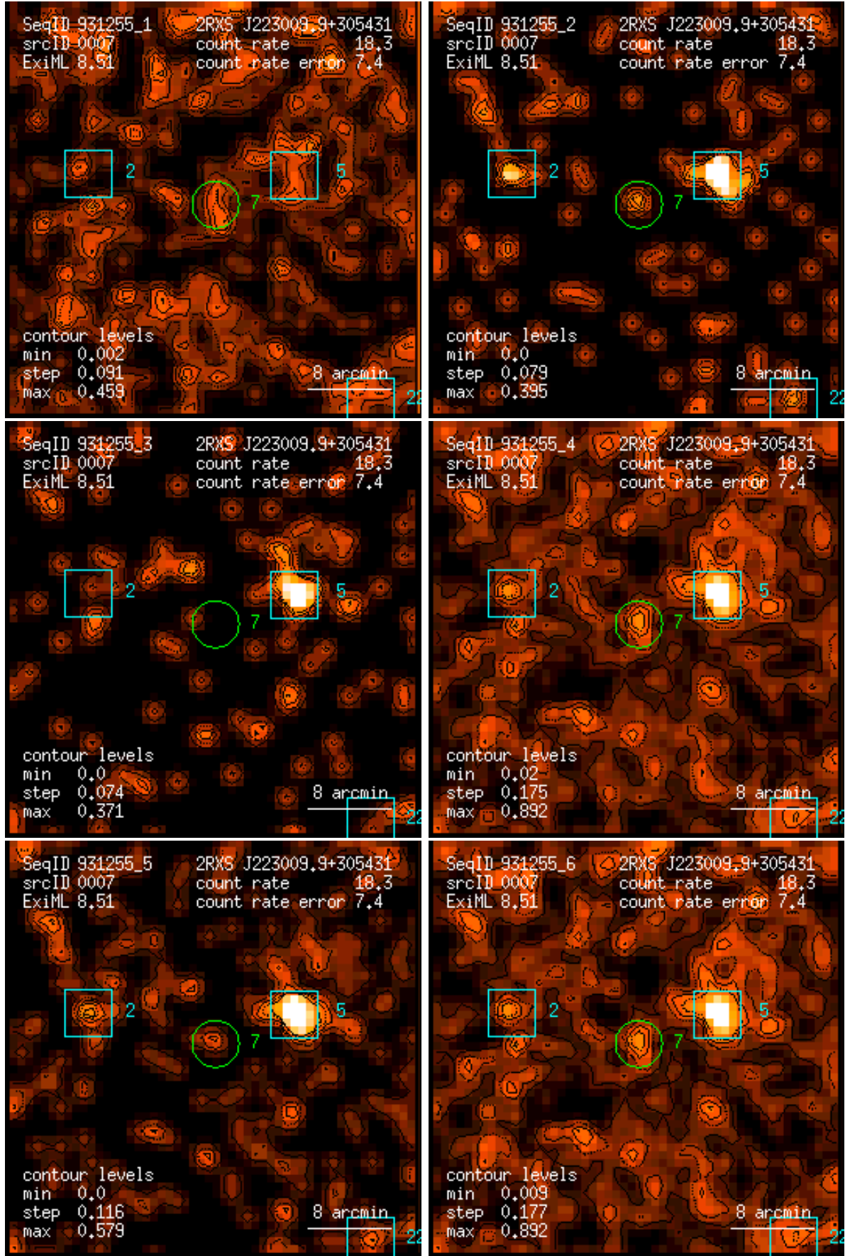
Figure 7: RASS 931255: detection 0007: band rate images, Gaussian filter: (1) PSPC channels 11 – 41, (2) 52 – 90, (3) 91 – 201, (4) 11 – 235, (5) 52 – 201, (6) 11 – 201. Broad band rates in counts/ks. Band rate contour levels in counts/ks/arcmin 2 .
