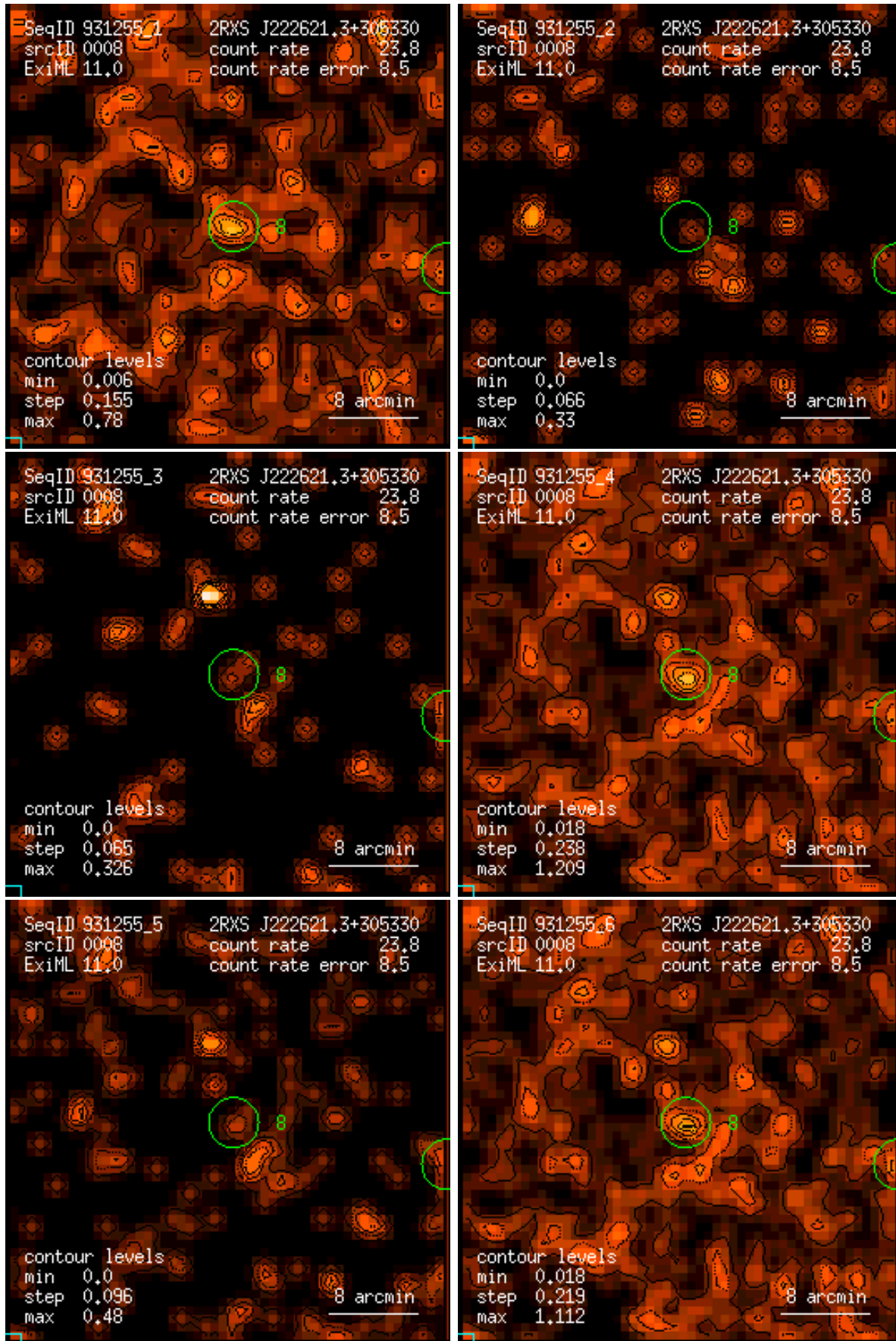
Figure 8: RASS 931255: detection 0008: band rate images, Gaussian filter: (1) PSPC channels 11 – 41, (2) 52 – 90, (3) 91 – 201, (4) 11 – 235, (5) 52 – 201, (6) 11 – 201. Broad band rates in counts/ks. Band rate contour levels in counts/ks/arcmin 2 .
