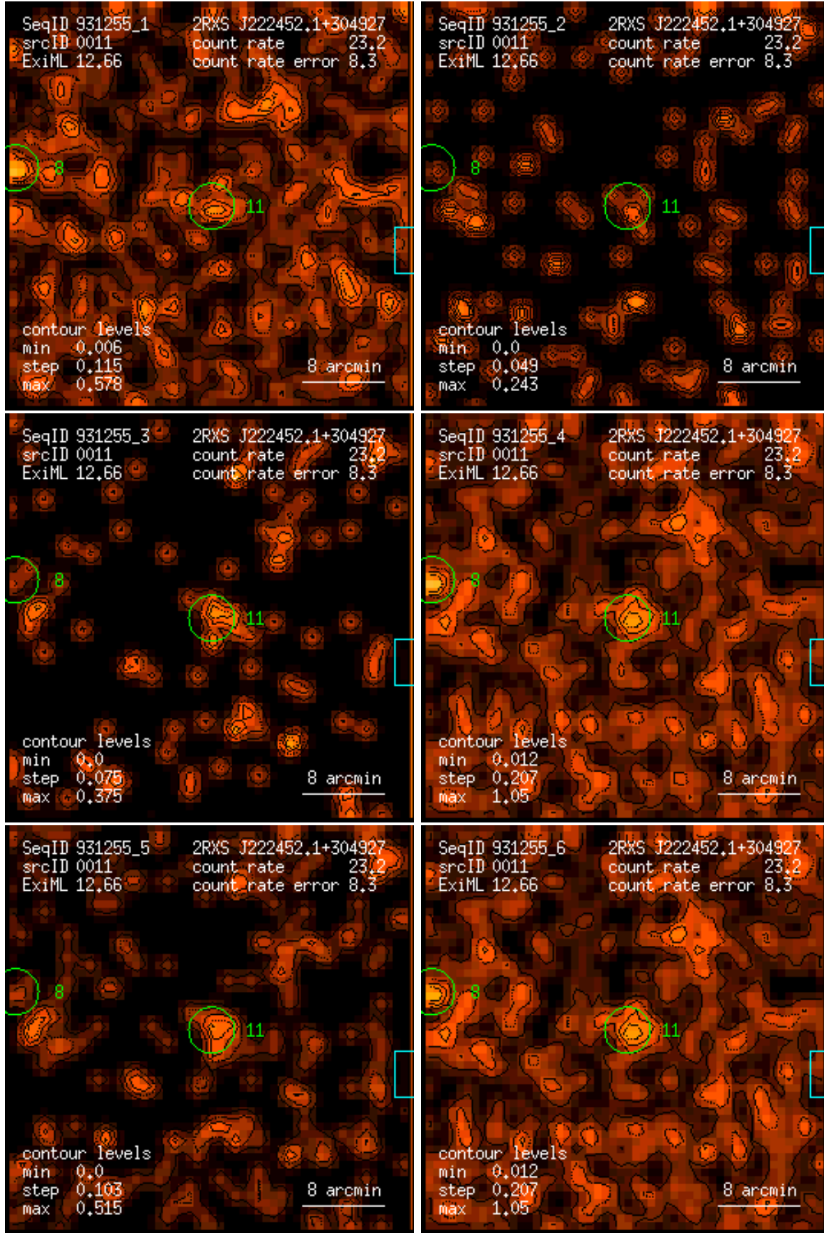
Figure 11: RASS 931255: detection 0011: band rate images, Gaussian filter: (1) PSPC channels 11 – 41, (2) 52 – 90, (3) 91 – 201, (4) 11 – 235, (5) 52 – 201, (6) 11 – 201. Broad band rates in counts/ks. Band rate contour levels in counts/ks/arcmin 2 .
