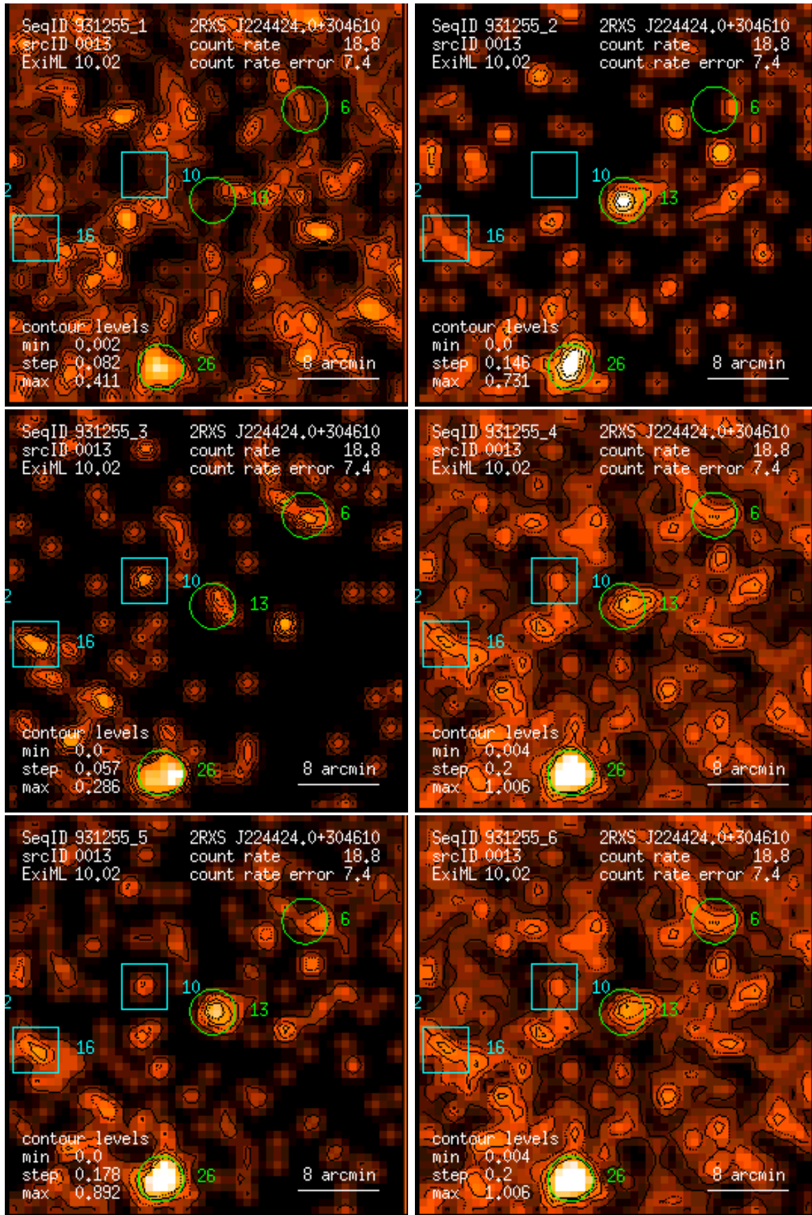
Figure 13: RASS 931255: detection 0013: band rate images, Gaussian filter: (1) PSPC channels 11 – 41, (2) 52 – 90, (3) 91 – 201, (4) 11 – 235, (5) 52 – 201, (6) 11 – 201. Broad band rates in counts/ks. Band rate contour levels in counts/ks/arcmin 2 .
