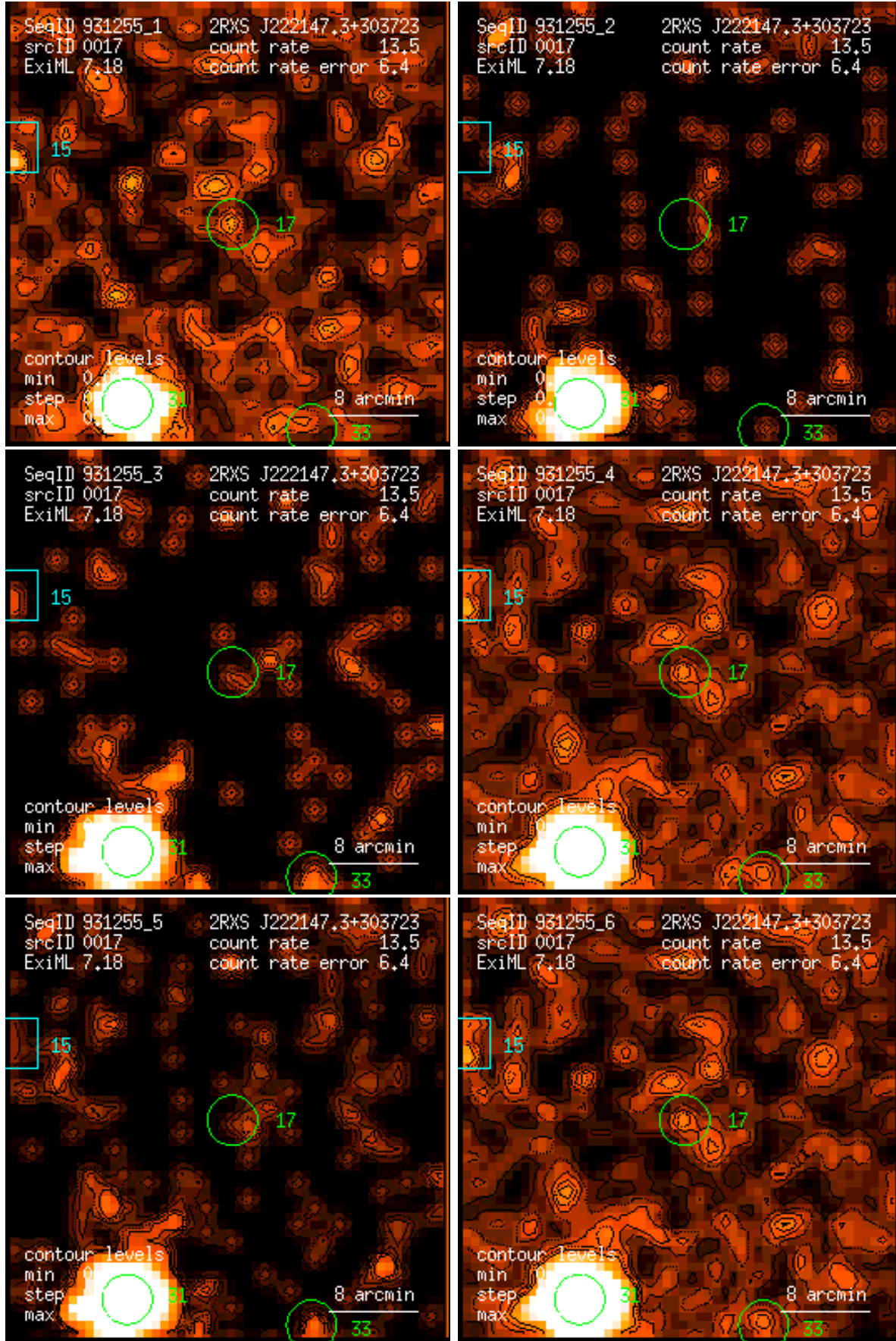
Figure 17: RASS 931255: detection 0017: band rate images, Gaussian filter: (1) PSPC channels 11 – 41, (2) 52 – 90, (3) 91 – 201, (4) 11 – 235, (5) 52 – 201, (6) 11 – 201. Broad band rates in counts/ks. Band rate contour levels in counts/ks/arcmin 2 .
