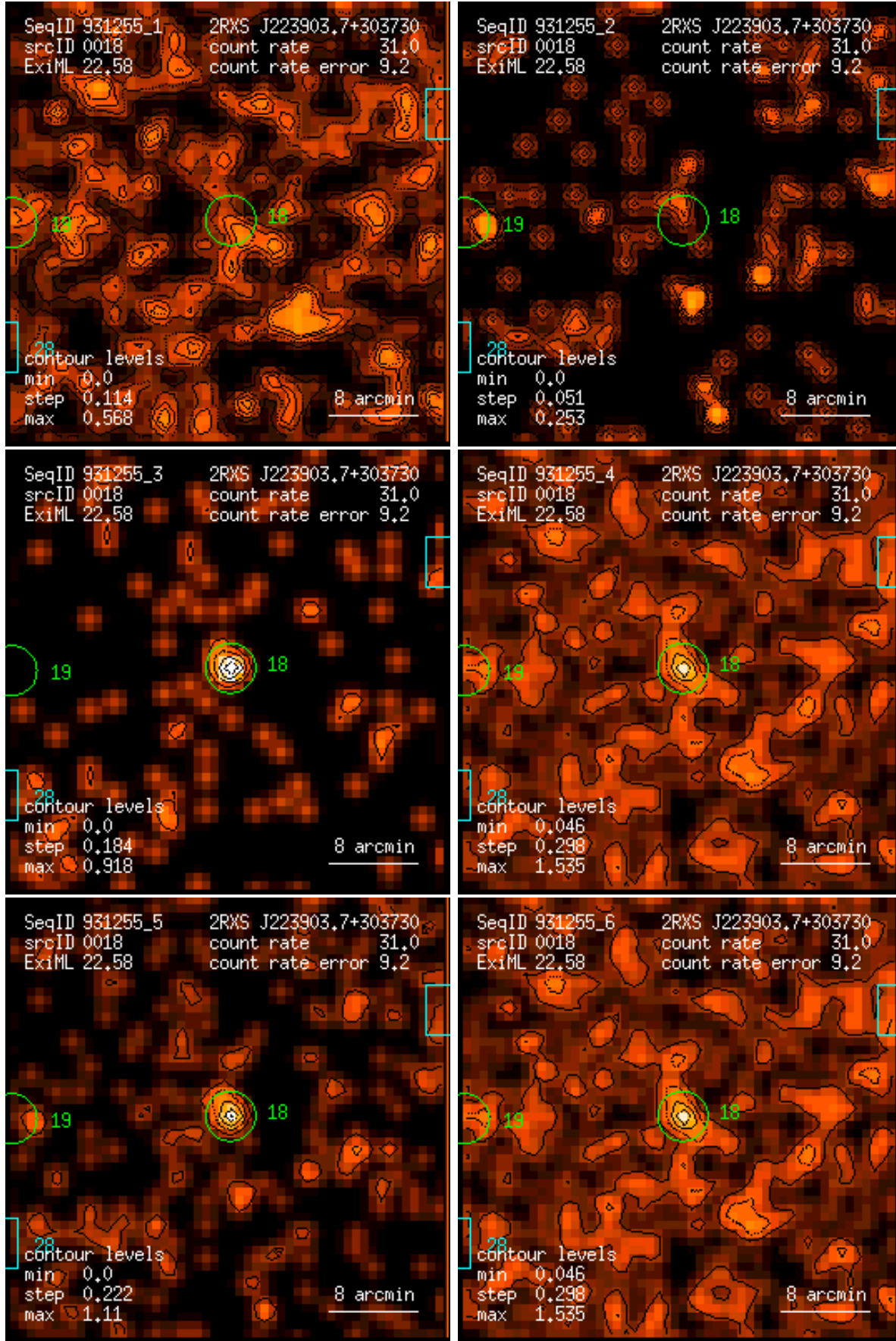
Figure 18: RASS 931255: detection 0018: band rate images, Gaussian filter: (1) PSPC channels 11 – 41, (2) 52 – 90, (3) 91 – 201, (4) 11 – 235, (5) 52 – 201, (6) 11 – 201. Broad band rates in counts/ks. Band rate contour levels in counts/ks/arcmin 2 .
