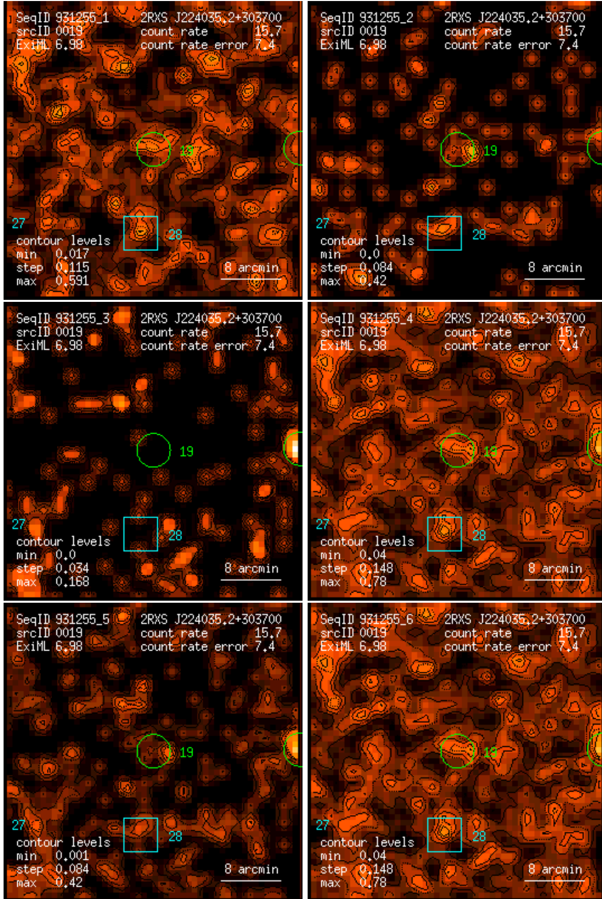
Figure 19: RASS 931255: detection 0019: band rate images, Gaussian filter: (1) PSPC channels 11 – 41, (2) 52 – 90, (3) 91 – 201, (4) 11 – 235, (5) 52 – 201, (6) 11 – 201. Broad band rates in counts/ks. Band rate contour levels in counts/ks/arcmin 2 .
