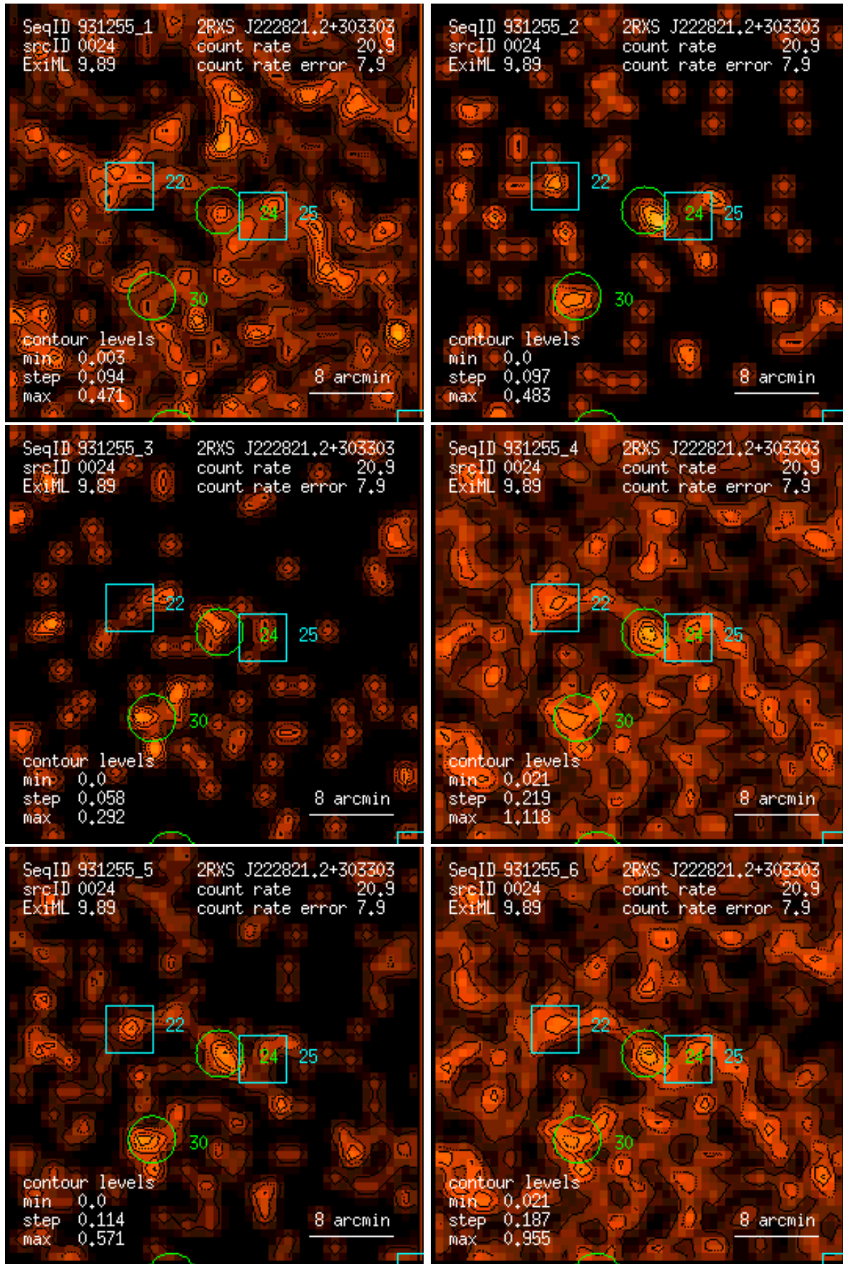
Figure 24: RASS 931255: detection 0024: band rate images, Gaussian filter: (1) PSPC channels 11 – 41, (2) 52 – 90, (3) 91 – 201, (4) 11 – 235, (5) 52 – 201, (6) 11 – 201. Broad band rates in counts/ks. Band rate contour levels in counts/ks/arcmin 2 .
