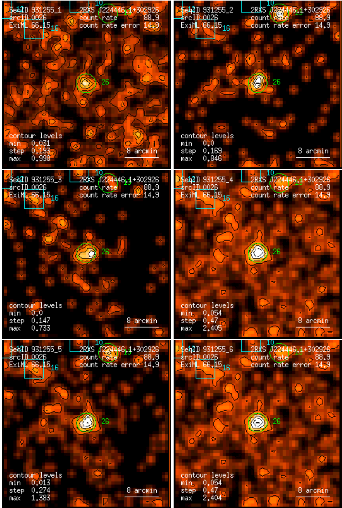
Figure 26: RASS 931255: detection 0026: band rate images, Gaussian filter: (1) PSPC channels 11 – 41, (2) 52 – 90, (3) 91 – 201, (4) 11 – 235, (5) 52 – 201, (6) 11 – 201. Broad band rates in counts/ks. Band rate contour levels in counts/ks/arcmin 2 .
