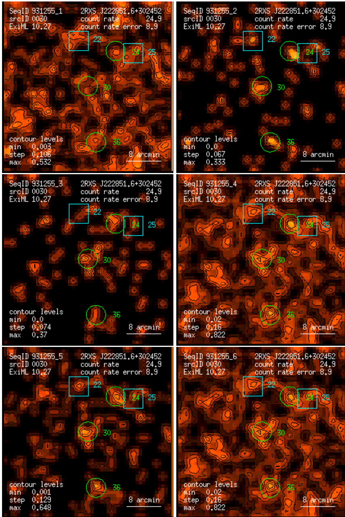
Figure 30: RASS 931255: detection 0030: band rate images, Gaussian filter: (1) PSPC channels 11 – 41, (2) 52 – 90, (3) 91 – 201, (4) 11 – 235, (5) 52 – 201, (6) 11 – 201. Broad band rates in counts/ks. Band rate contour levels in counts/ks/arcmin 2 .
