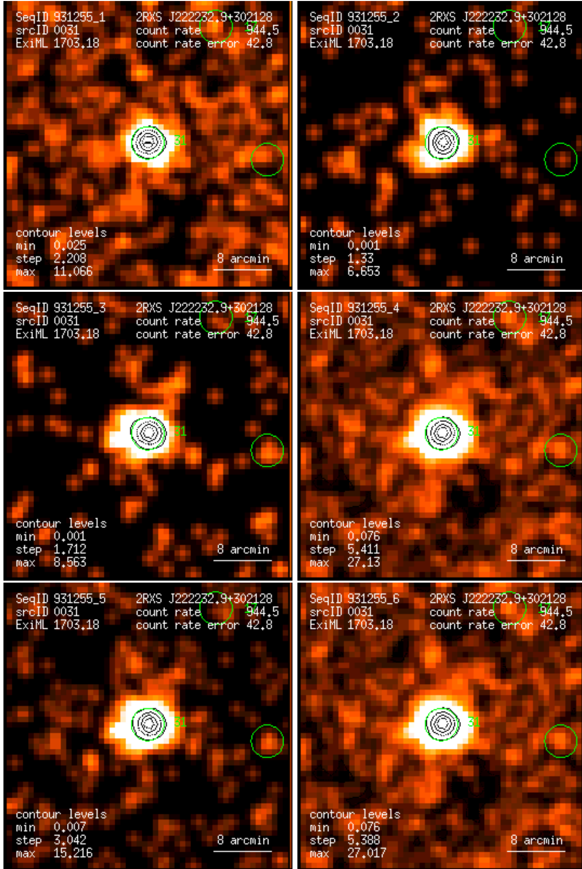
Figure 31: RASS 931255: detection 0031: band rate images, Gaussian filter: (1) PSPC channels 11 – 41, (2) 52 – 90, (3) 91 – 201, (4) 11 – 235, (5) 52 – 201, (6) 11 – 201. Broad band rates in counts/ks. Band rate contour levels in counts/ks/arcmin 2 .
