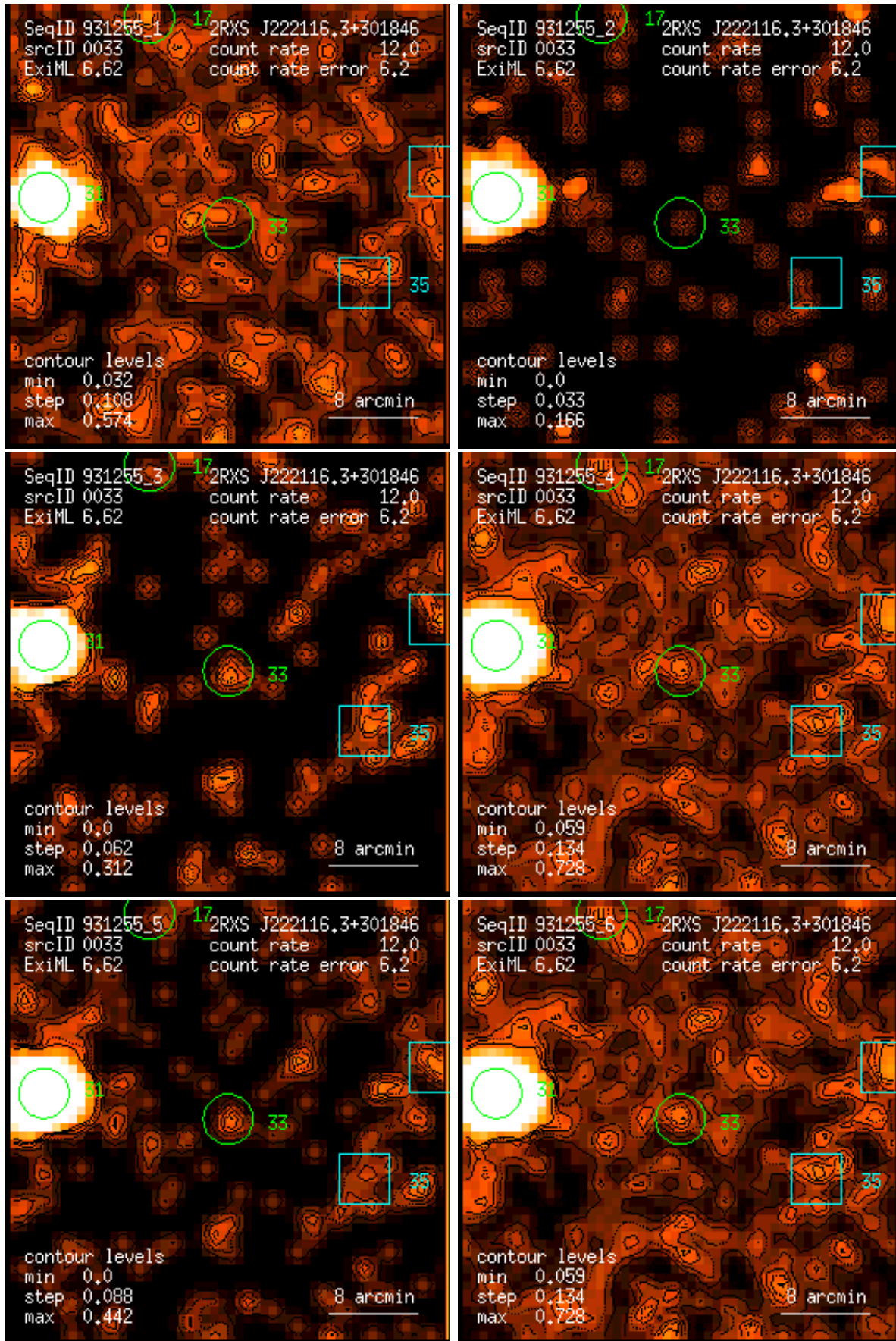
Figure 33: RASS 931255: detection 0033: band rate images, Gaussian filter: (1) PSPC channels 11 – 41, (2) 52 – 90, (3) 91 – 201, (4) 11 – 235, (5) 52 – 201, (6) 11 – 201. Broad band rates in counts/ks. Band rate contour levels in counts/ks/arcmin 2 .
