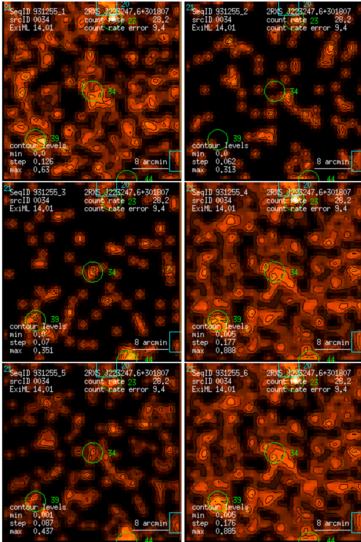
Figure 34: RASS 931255: detection 0034: band rate images, Gaussian filter: (1) PSPC channels 11 – 41, (2) 52 – 90, (3) 91 – 201, (4) 11 – 235, (5) 52 – 201, (6) 11 – 201. Broad band rates in counts/ks. Band rate contour levels in counts/ks/arcmin 2 .
