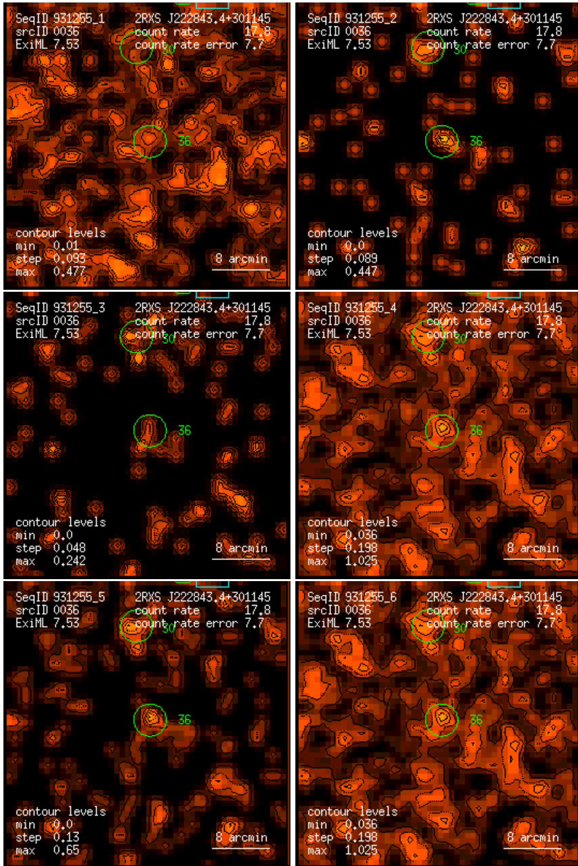
Figure 36: RASS 931255: detection 0036: band rate images, Gaussian filter: (1) PSPC channels 11 – 41, (2) 52 – 90, (3) 91 – 201, (4) 11 – 235, (5) 52 – 201, (6) 11 – 201. Broad band rates in counts/ks. Band rate contour levels in counts/ks/arcmin 2 .
