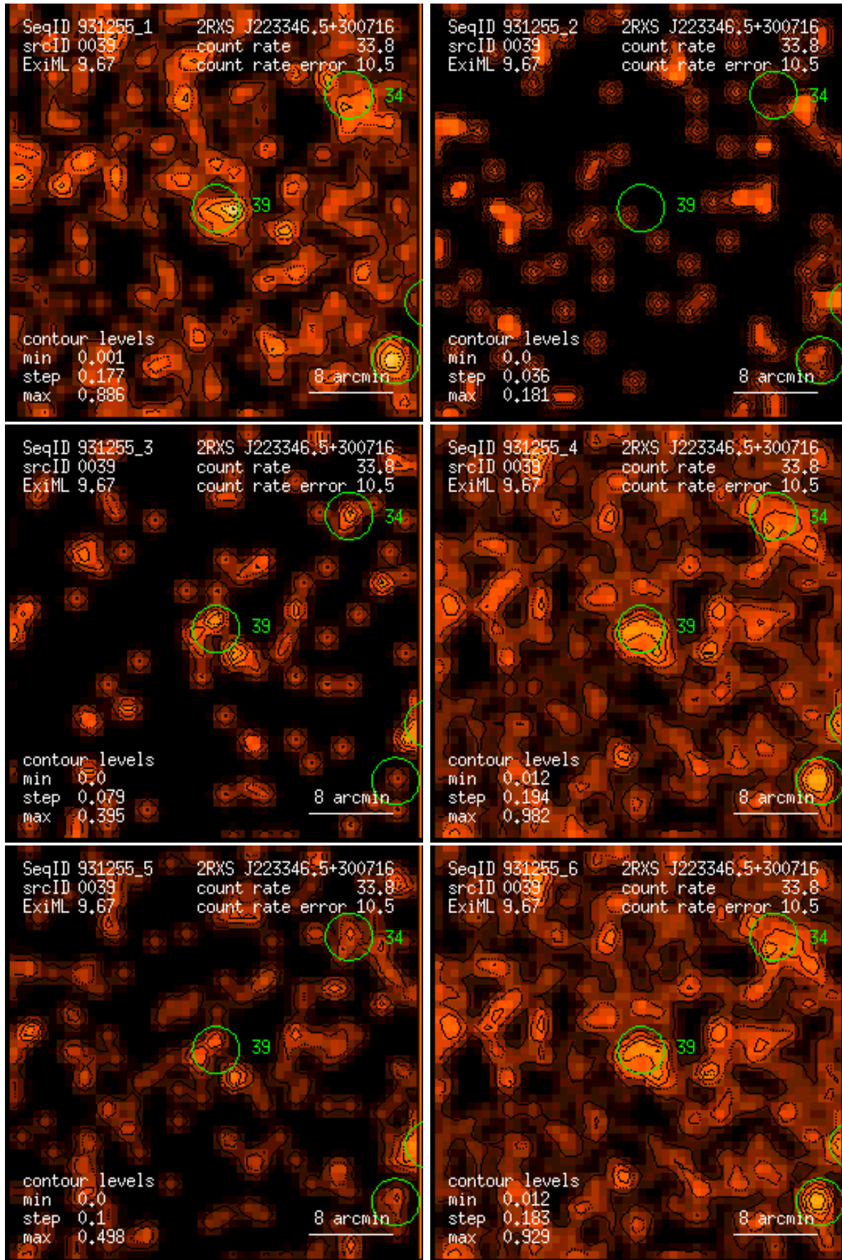
Figure 39: RASS 931255: detection 0039: band rate images, Gaussian filter: (1) PSPC channels 11 – 41, (2) 52 – 90, (3) 91 – 201, (4) 11 – 235, (5) 52 – 201, (6) 11 – 201. Broad band rates in counts/ks. Band rate contour levels in counts/ks/arcmin 2 .
