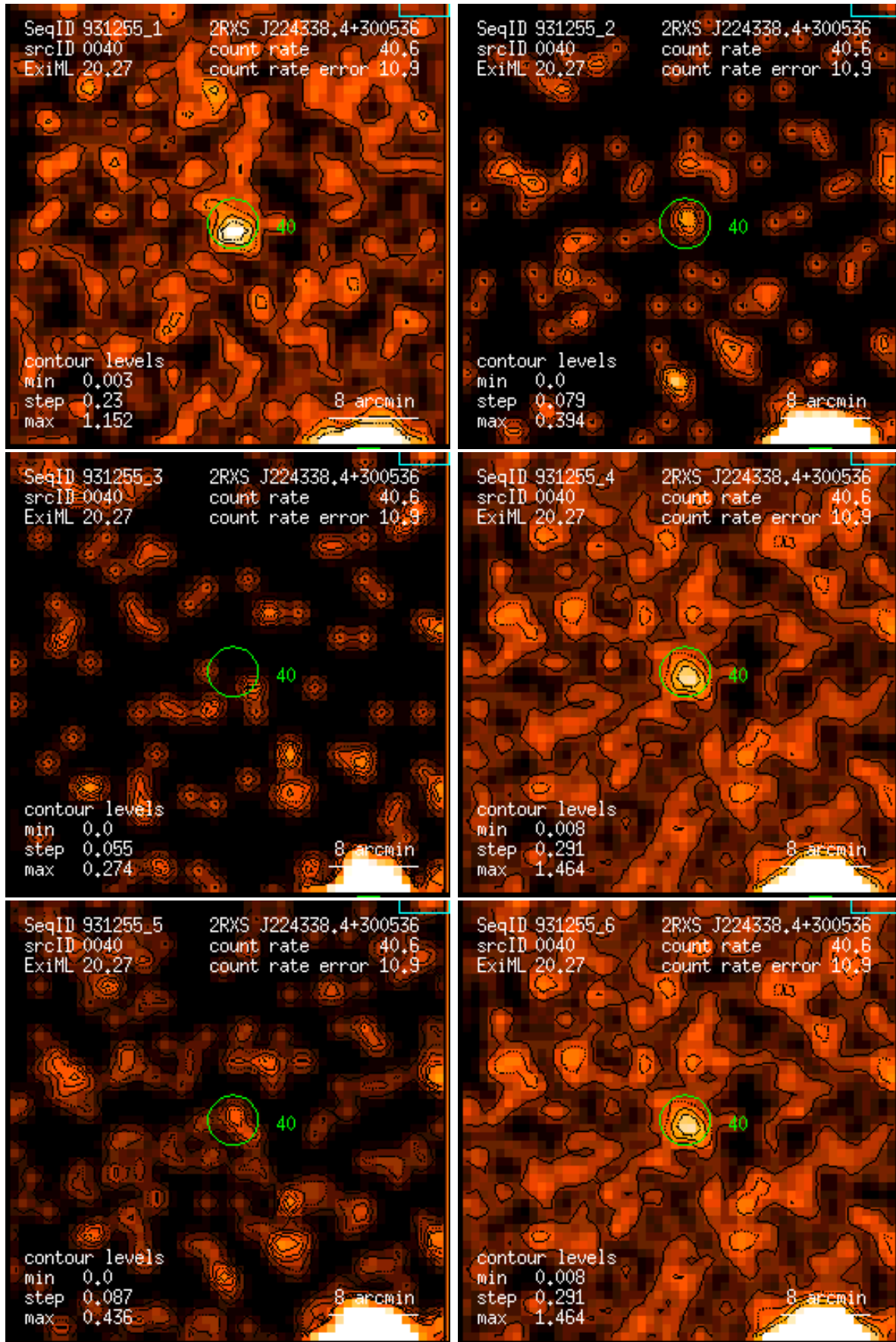
Figure 40: RASS 931255: detection 0040: band rate images, Gaussian filter: (1) PSPC channels 11 – 41, (2) 52 – 90, (3) 91 – 201, (4) 11 – 235, (5) 52 – 201, (6) 11 – 201. Broad band rates in counts/ks. Band rate contour levels in counts/ks/arcmin 2 .
